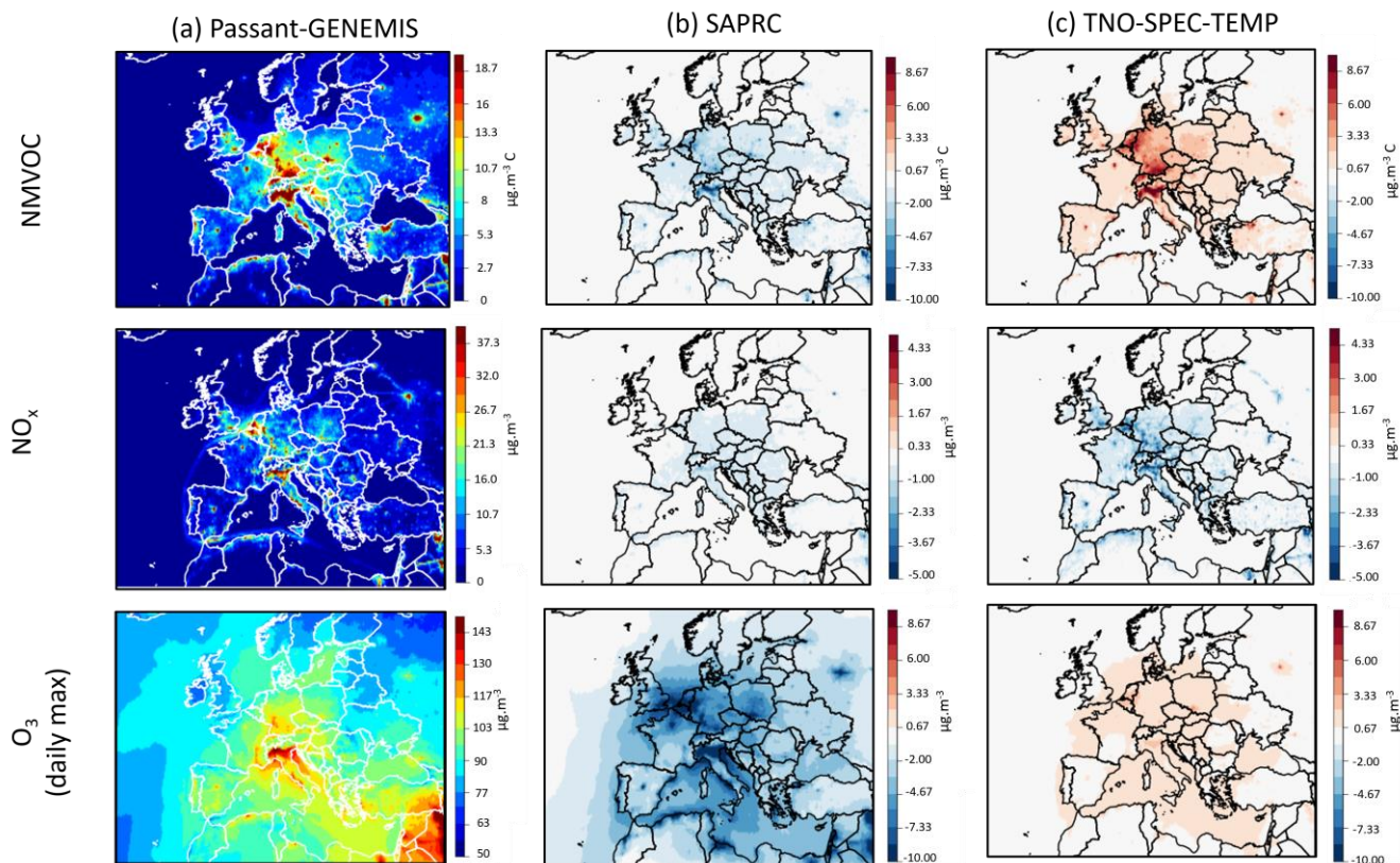
Figure 10. (a) Reference NMVOC, NO x and O 3 concentrations ( \mu\text{g}/\text{m}^3 ) (Passant-GENEMIS) and absolute difference between (b) SAPRC and Passant-GENEMIS concentrations and (c) TNO-SPEC-TEMP and Passant-GENEMIS concentrations. Concentrations are averaged over the period of June 2018–August 2018 for daily mean values (NMVOC and NO x ) and daily max values (O 3 ).
