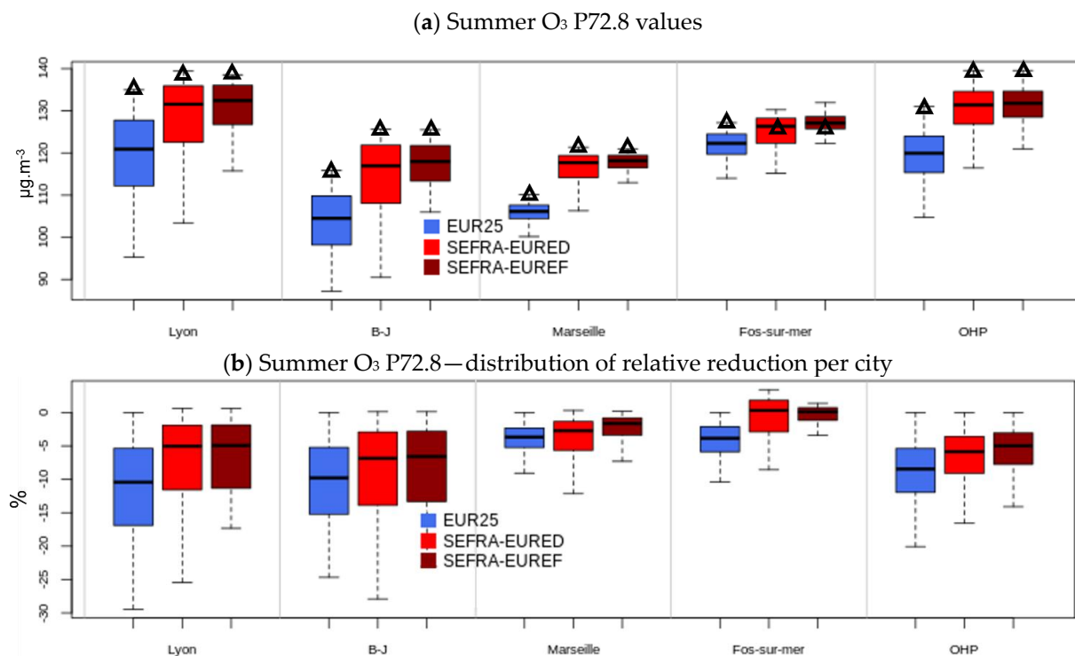
Figure 5. Distribution of summer O 3 P72.8 per city: Top (a): P72.8 values when emissions for both the industrial and the road transport sector are reduced between 0 and 100% by increments of 1%, and reference O 3 P72.8 value (triangle) where no reduction is applied. Bottom (b): distribution of O 3 P72.8 difference (in %) between the scenario where emissions are reduced and the reference without emission reductions. Blue: EUR25. Red: SEFRA04-EURED. Brown: SEFRA-EUREF.
