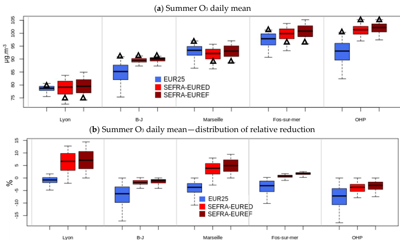
Figure 7. Distribution of the summer average of the O 3 daily mean per city: Top (a): O 3 daily mean values (in µg/m 3 ) when emissions for both the industrial and the road transport sector are reduced between 0 and 100% by increments of 1%, and reference O 3 value (triangle) where no reduction is applied. Bottom (b): distribution of O 3 daily mean difference (in %) between the scenario where emissions are reduced and the reference without emission reductions. Blue: EUR25. Red: SEFRA04-EURED. Brown: SEFRA-EUREF.
