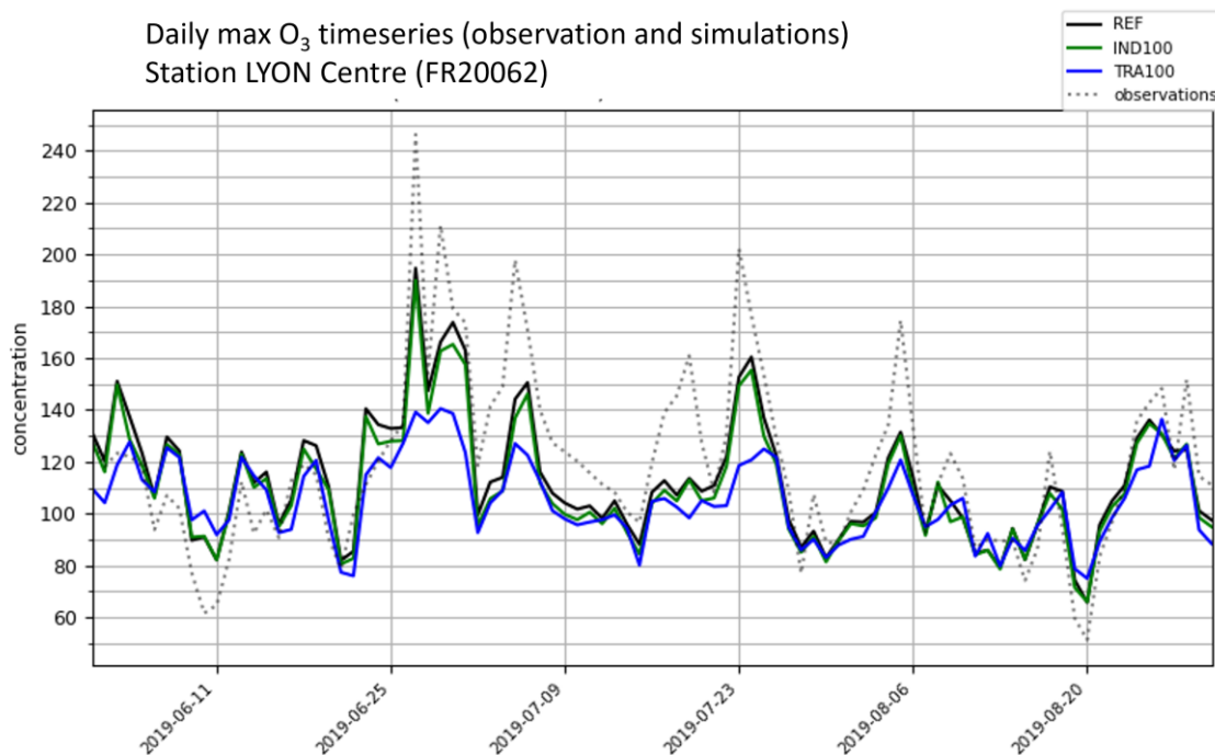
Figure 8. Time-series of O 3 daily max SEFRA04 (-EURED) simulation for the reference simulation (black line—no emission reductions), traffic 100% reduction (TRA100, blue line), industrial 100% reduction (IND100, green line) scenario and observations (dotted grey line) for Lyon station FR20062 during summer 2019.
