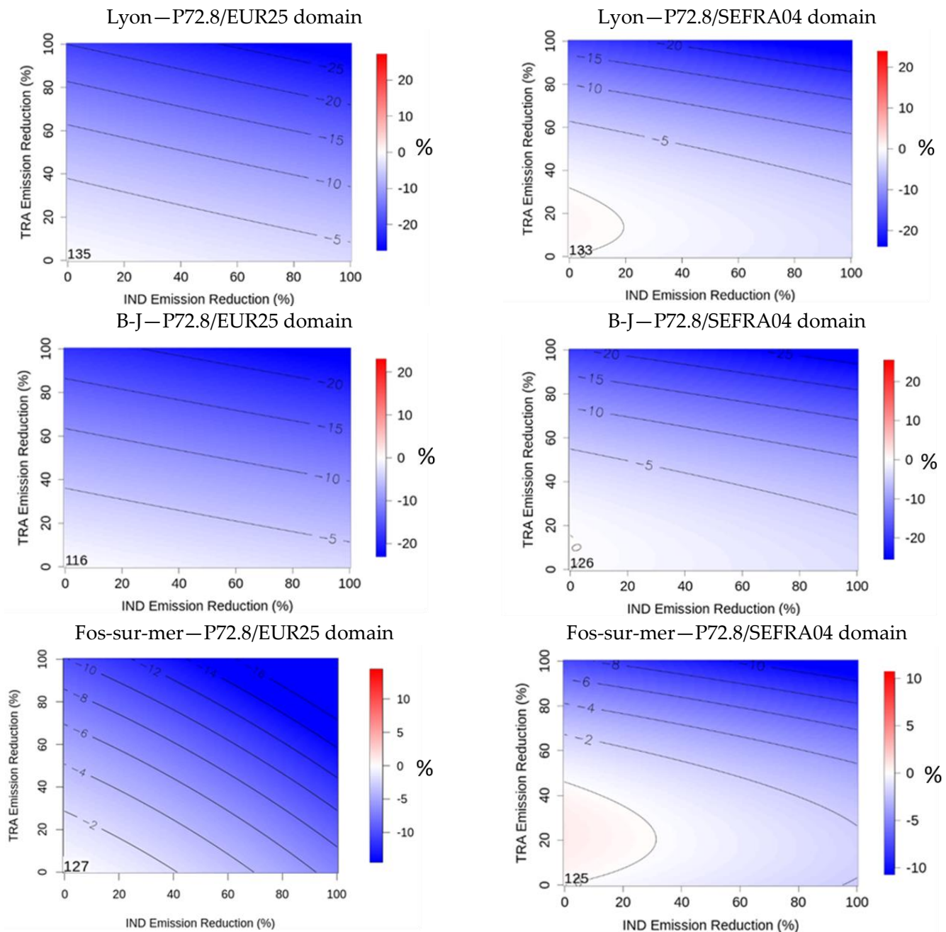
Figure 4. Summer O 3 P72.8 response in % (negative changes, blue, for a decrease) corresponding to a given reduction in Traffic (TRA) and Industry (IND) emissions over Lyon ( top panel), B-J ( middle panel) and Fos-sur-mer ( bottom panel). Results for the EUR25 resolution are shown on the ( left ), and for the SEFRA04 resolution on the ( right ). Both used BC-EURED (Boundary Conditions with REDuction over Europe). The absolute O 3 concentrations for the summer P72.8 in the reference simulation (when no reduction is applied) are displayed at the bottom left corner (in \mu\text{g}/\text{m}^3 ).
