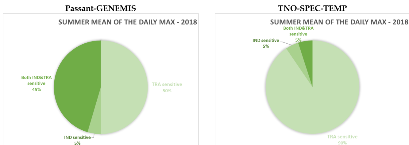
Figure 12. Classification of ozone regimes for ozone daily maxima averaged over the summer 2018 for the 22 target cities used in [13]. (Left): ACT results trained on CHIMERE setup based on Passant-GENEMIS. (Right): ACT results trained on CHIMERE setup based on TNO-SPEC-TEMP.
