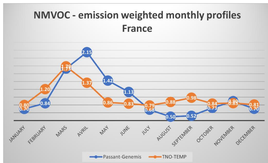
Figure A2. Emission-weighted monthly profiles for NMVOCs as used for France in CHIMERE.
