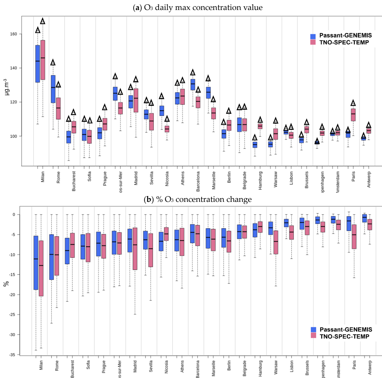
Figure 11. Distribution of O_3 daily maxima over the summer 2018 for 22 cities in Europe. Top (a): absolute concentrations when emissions for both the industrial and the road transport sector are reduced between 0 and 100% by increments of 1%, and reference O_3 value (triangle) where no reduction is applied. Bottom (b): distribution of the concentration difference (in %) between the scenario where emissions are reduced and the reference without emission reductions. Blue: Passant-GENEMIS, pink: TNO-SPEC-TEMP. Negative values mean reduction in O_3 consecutive to emission reductions.
