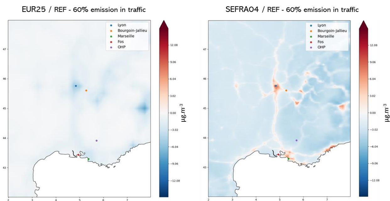
Figure 3. Difference in summer average daily mean O 3 concentrations (µg/m 3 ) between the reference simulation (no emission reductions) and a scenario where traffic emissions are reduced by 60% uniformly. Results for the EUR25 domain (25 km × 25 km resolution) are shown on the left , and for the SEFRA04 domain (4 km × 4 km resolution) in the right panel.
