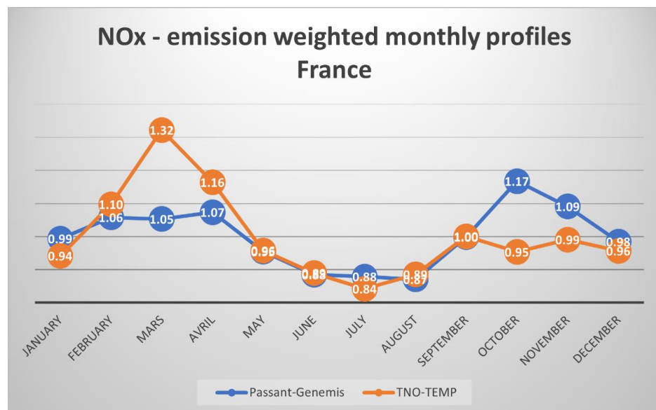
Figure A1. Emission-weighted monthly profiles for NO x as used for France in CHIMERE.
