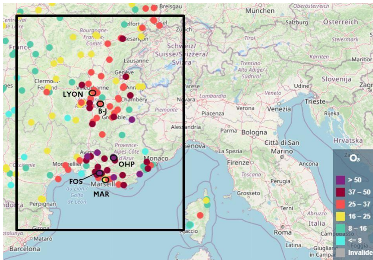
Figure 1. Annual number of O 3 exceedances of the 120 \mu\text{g}/\text{m}^3 threshold for the maximum daily eight-hour mean in 2019. Maximum number of exceedances for the EU's current target value is fixed at 25 days. This also corresponds to the percentile 93.15, which should not exceed 120 \mu\text{g}/\text{m}^3 . The black rectangle characterises the SEFRA domain. The 5 stations used for analyses are highlighted with black circles.
