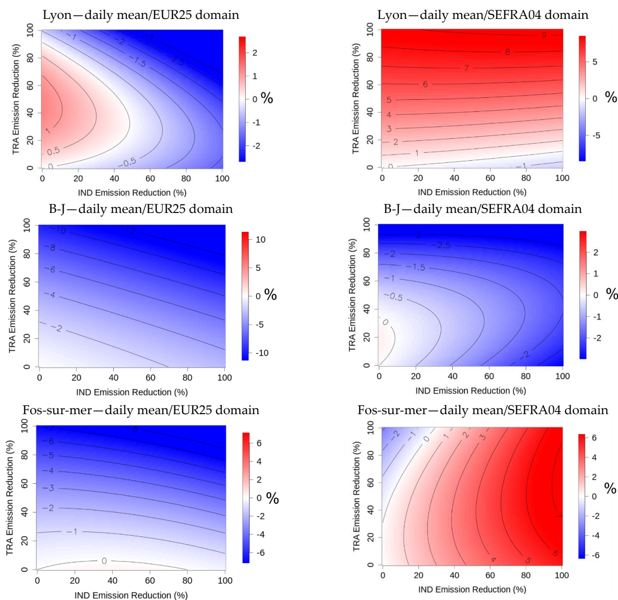
Figure 6. Summer average of the O 3 daily mean: response in % (negative for a decrease in blue) corresponding to a given reduction in Traffic and Industry emissions over Lyon ( top panel), B-J ( middle panel) and Fos-sur-mer ( bottom panel). Results for the EUR25 resolution are shown on the ( left ), and for the SEFRA04 resolution on the ( right ). Both used BC-EURED (Boundary Conditions with REDuction over Europe).
