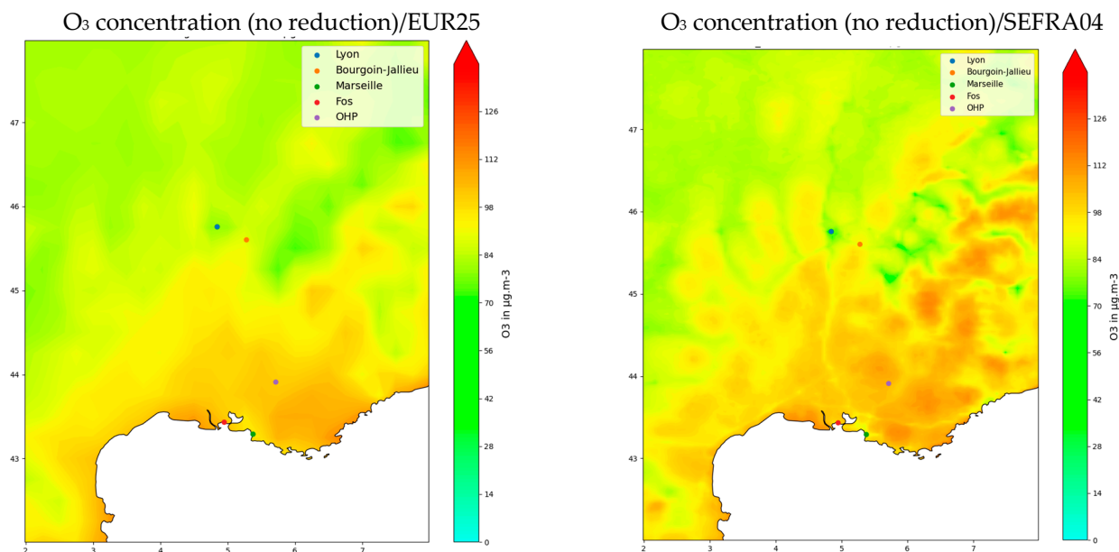
Figure 2. NO 2 average emissions in Tonnes/km 2 (top) and daily mean O 3 concentration (bottom) averaged over summer 2019 (JJA—June, July, August) simulated with no emission reductions for EUR25 resolution (25 km × 25 km) (left) and SEFRA04 resolution (4 km × 4 km) (right).
