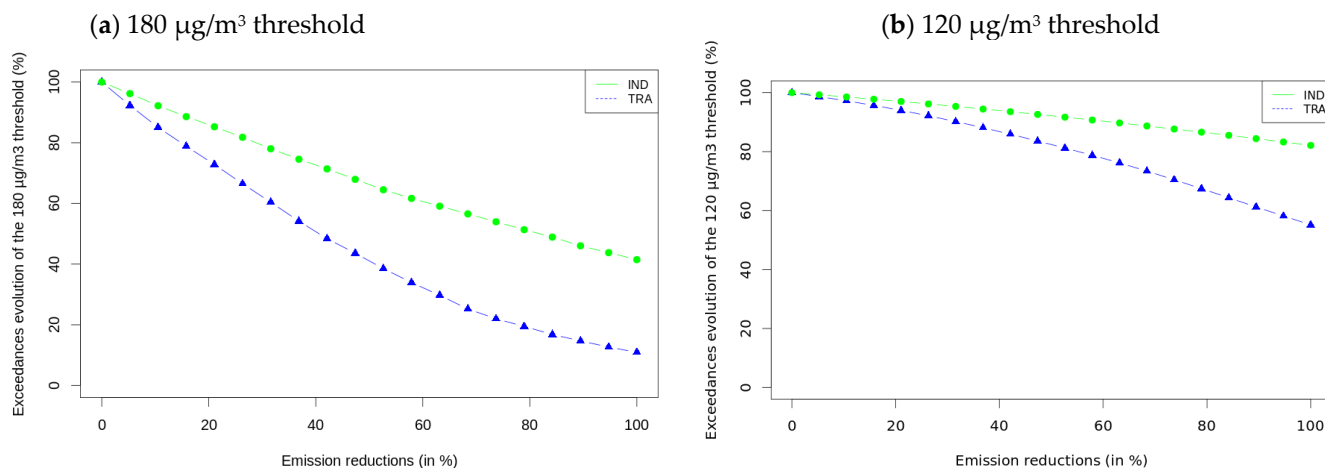
Figure 9. Evolution of the number of grid cells of the SEFRA04 region in exceedances of the (a) 180 \mu\text{g}/\text{m}^3 and (b) 120 \mu\text{g}/\text{m}^3 thresholds, respectively, as simulated with emission reduction from the Traffic (TRA) sector (blue line) and the Industrial (IND) sector (green line) ranging from 0 to 100%.
