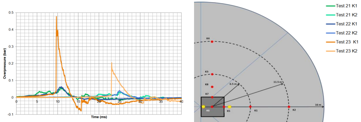
Figure 6. Overpressure comparison for the repeated trials 21 to 23 [34].
