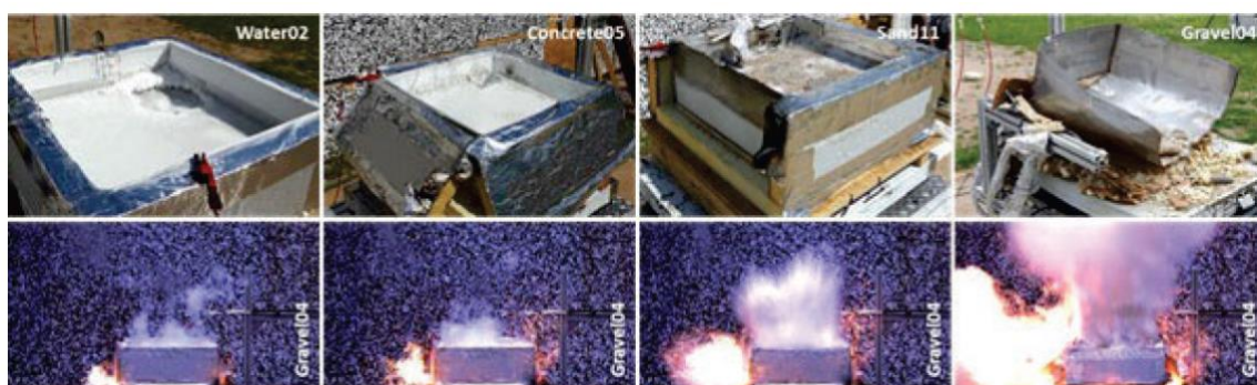
Figure 3 Different degrees of damage to the facility observed in the ignited pool experiments for the different substrates (upper row) and High-Speed video sequence of the final combustion event in experiment Gravel04 (2000 fps, lower row) [21].
