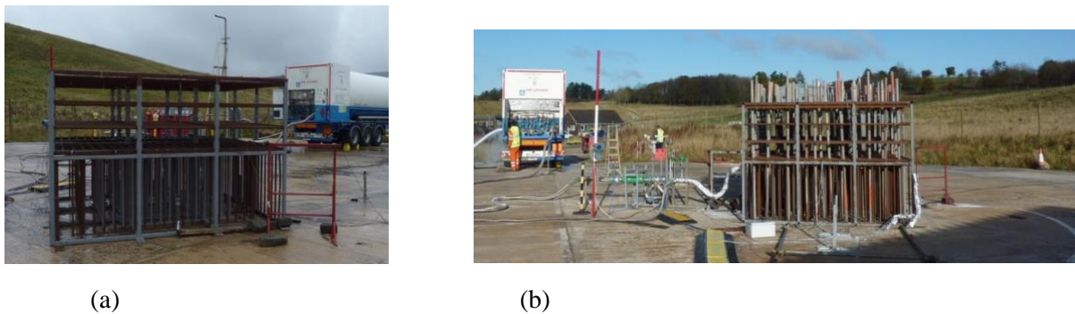
Figure 4. The tests rig used for the ignited tests with congestion and confinement (a) and additional congestion by scaffold poles (b). [34].
