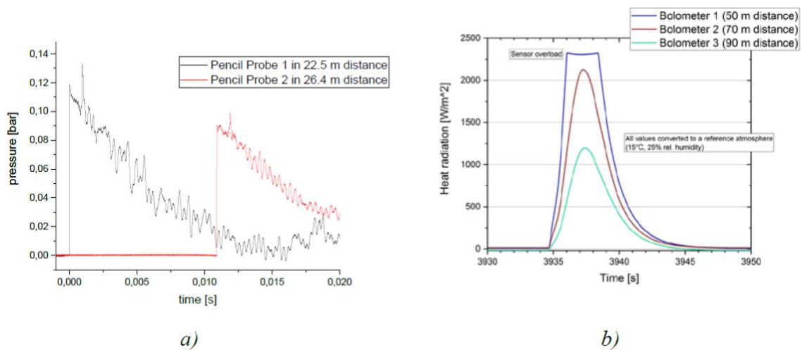
Figure 7. Overpressure and thermal radiation after the failure of an MLI-insulated vessel positioned horizontally filled with LH 2 (a) Blast waves measured at distances of 22.5 m and 26.4 m; (b) heat radiation from the burst of the MLI-insulated vessel [25,26].
