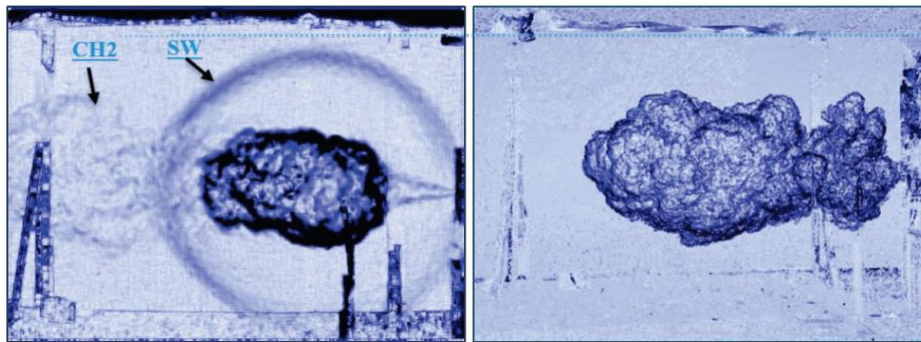
Figure 1. Shock wave formation (left) and a stationary jet fire (right) established under ignition of 4-mm nozzle and 20 MPa pressure hydrogen release: SW –shock wave; CH2 –unignited hydrogen [21].
