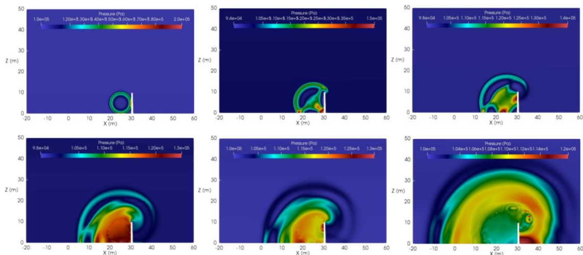
Figure 9. Predicted contours of pressure in the middle plane for the case of IR10 at a time sequence of 10 ms, 20 ms, 30 ms, 50 ms, 60 ms, 100 ms after the ignition.
