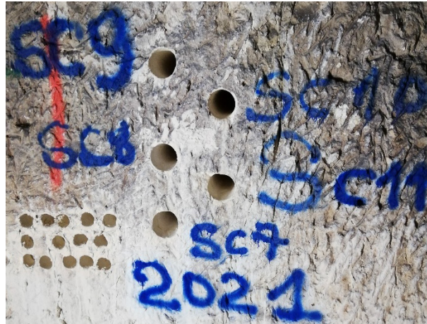
Figure 1. Plugs cored from pillars in the Royer mine.
