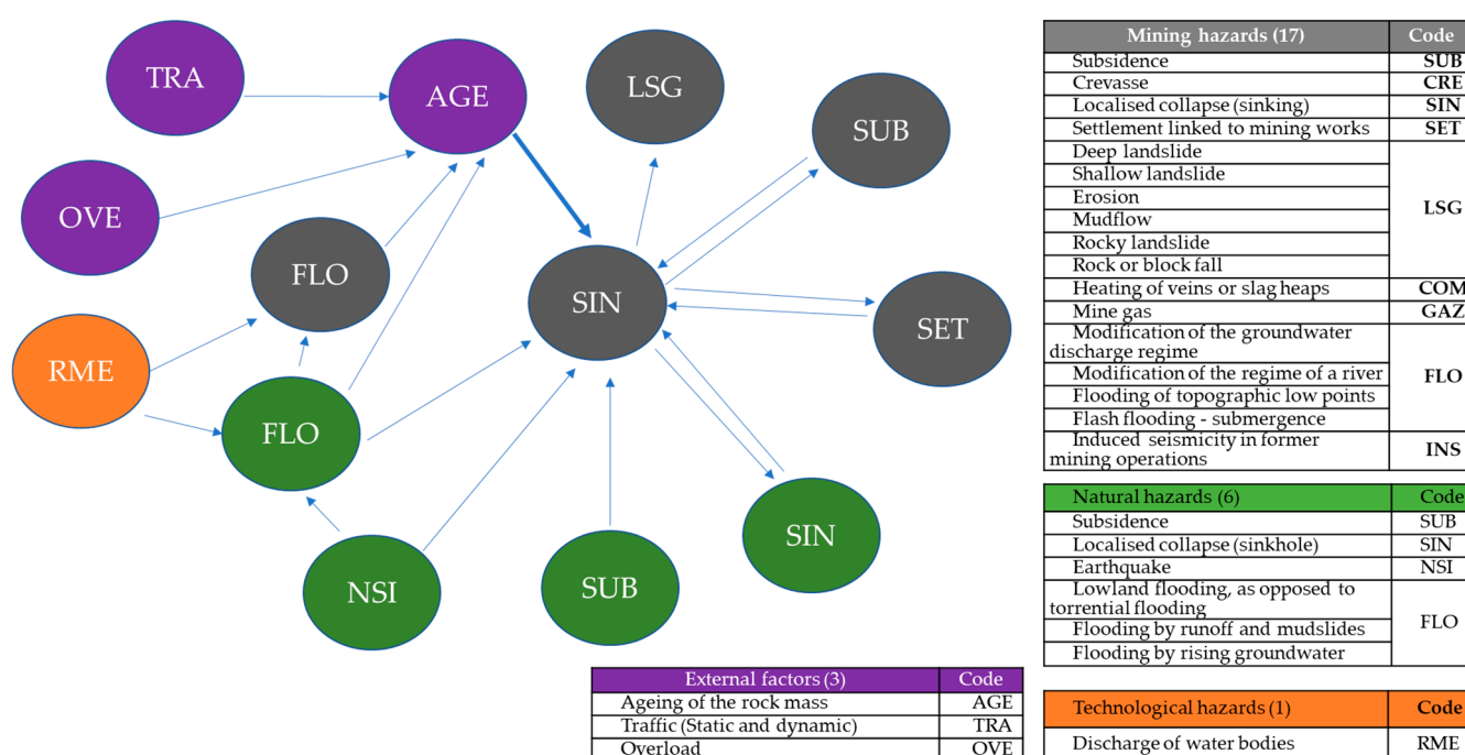
Figure 3. Examples of mining, natural, and technology hazards interaction.
