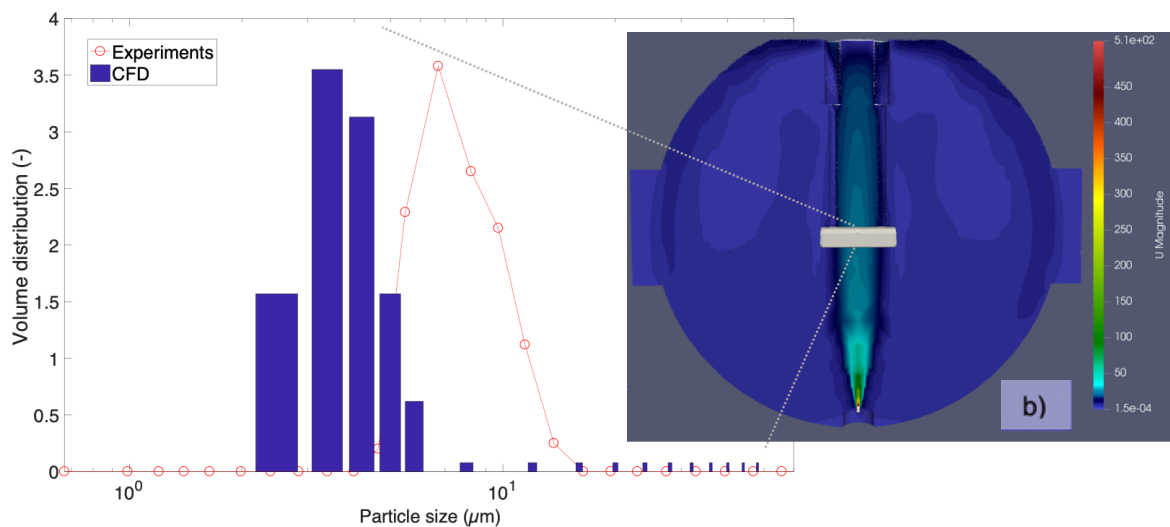
Figure 5: Comparison between CFD results and the experimental kerosene DSD at the sphere center after 1.5 s generation
