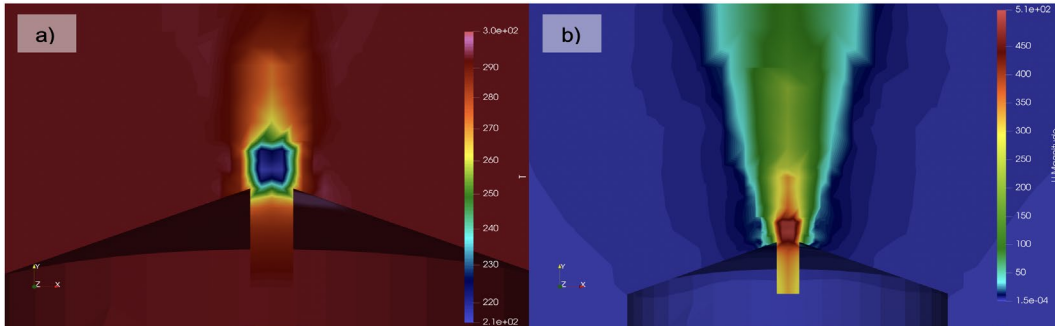
Figure 4: Representation of a) temperature and b) velocity iso-contour lines at the nozzle
