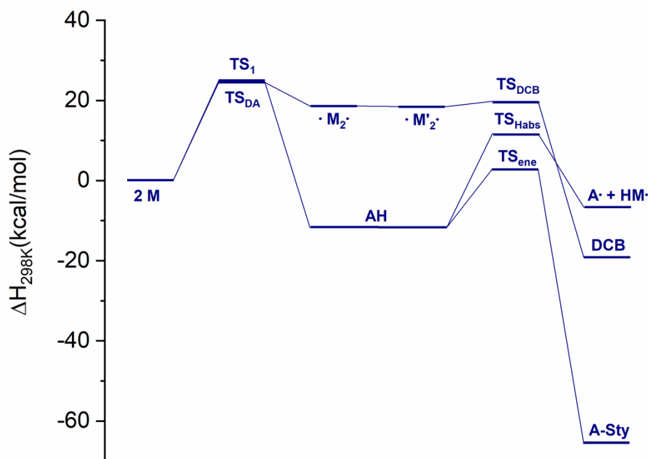
Figure 3: Energetic profile of the mechanisms involved and in competition with the initiation of styrene thermal polymerization, as calculated at M05-2X/6-31+G(d,p) level (Fayet and Rotureau, 2022)
