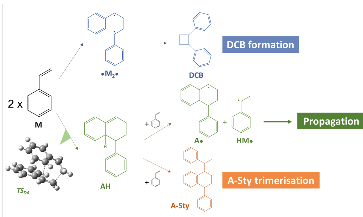
Figure 2: Reaction mechanisms involved and in competition with the initiation of styrene thermal polymerization, as proposed by Khuong (2005)
