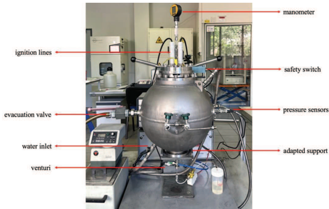
Figure 3: The Modified 20 L Ignition and explosion Severity Test device
