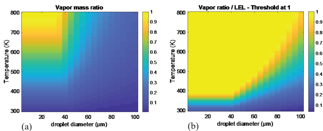
Figure 17: (a) the vapor mass ratio (b) the vapor/LEL ratio as a function of the initial temperature and droplet size for a 4 g Jet A1 mist cloud with a 1 ms delay
