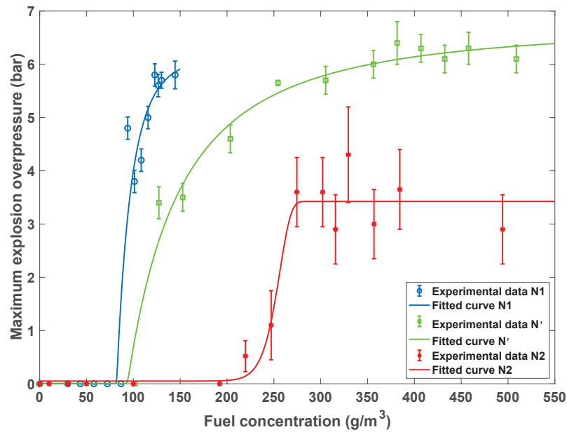
Figure 12: Variation of the maximum explosion overpressure as a function of Jet A1 mist concentrations for nozzle sets N1, N', and N2
