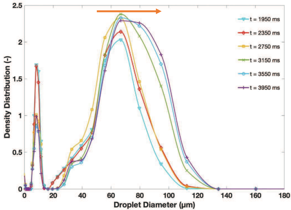
Figure 8: Droplet size volume / mass distribution of Jet A1 mists generated at P = 3 bar using nozzle set N2 - time step 400 ms starting from t_{inj} = 1950 ms
