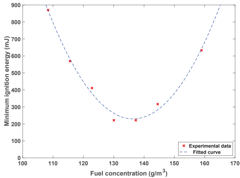
Figure 18: Variation of the minimum ignition energy with Jet A1 mist concentration at T = 27^\circ\text{C}
