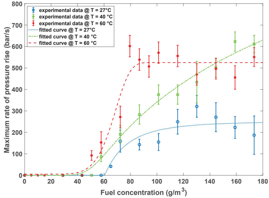
Figure 15: Variation of the maximum rate of pressure rise as a function of Jet A1 mist concentration at T = 27, 40 and 60\text{ }^{\circ}\text{C}
