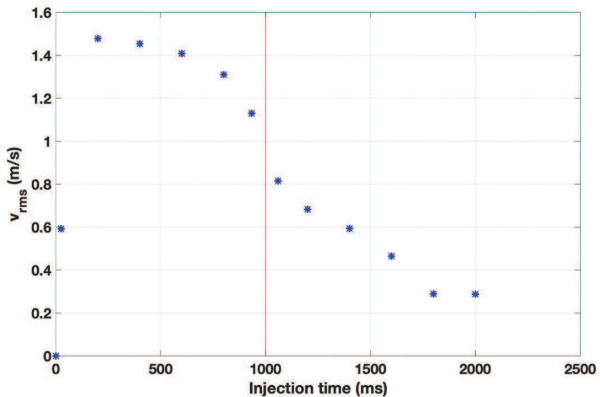
Figure 10: Evolution of the root-mean-square velocity with the mist injection time - generation using nozzle set N1 and P_{inj} = 3 bar
