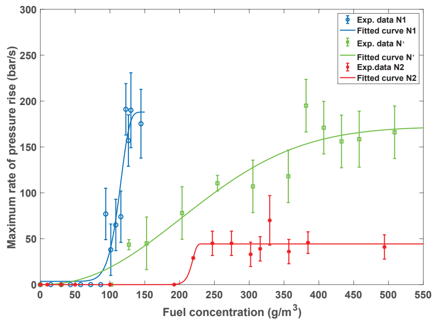
Figure 13: Variation of the maximum rate of pressure rise as a function of Jet A1 mist concentrations for nozzle sets N1, N', and N2
