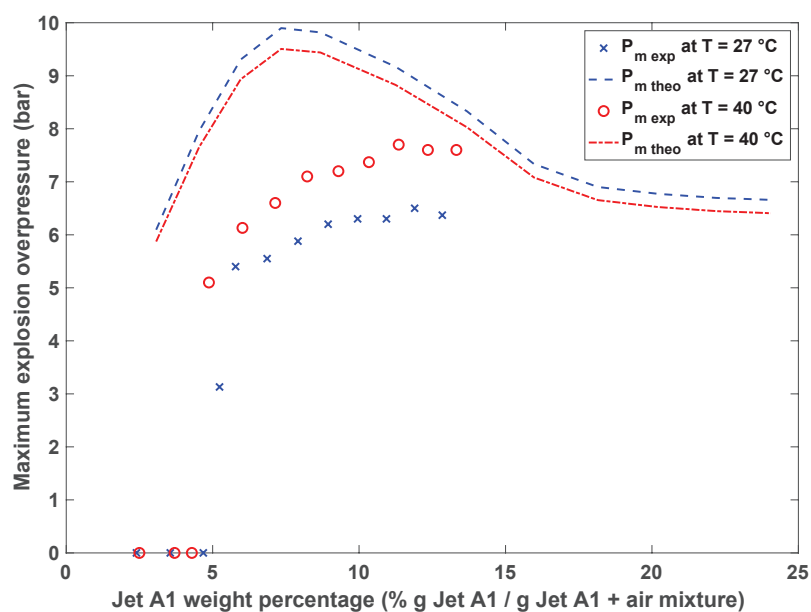
Figure 16: Comparison of theoretical adiabatic explosion overpressure and experimental results for Jet A1 mists at T = 27 and 40 °C
