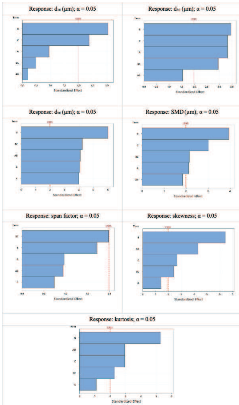
Figure 9: Pareto Charts of the Standardized Effects for d_{10} , d_{50} , d_{90} , SMD, span factor, skewness, and kurtosis (Factors A = orifice diameter, B = air injection pressure, C = fluid
