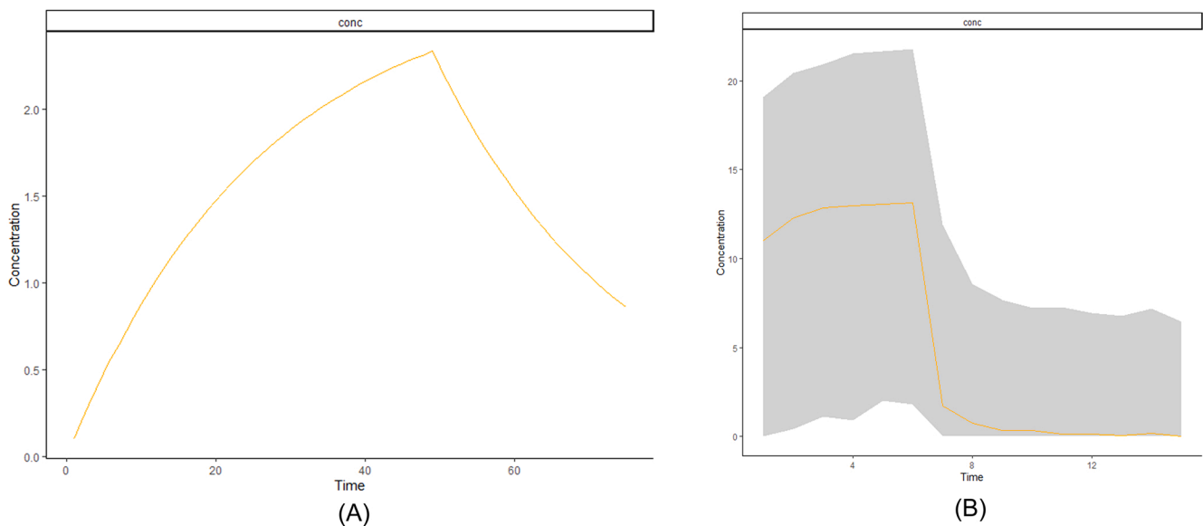
Fig. 5. Example of a prediction step for (A) fish Oncorhynchus mykiss exposed to a hydrophobic chemical and (B) Spirostomum ambiguum exposed to fluoxetine. The orange curve is the predicted median curve of the internal concentration predicted from the median TK parameter values provided in the original paper at 0.01 \mu\text{g mL}^{-1} (Crookes and Brooke, 2011) for (A) and at 0.025 \mu\text{g mL}^{-1} for (B) (Nalecz-Jaweski et al., 2020). The grey area is the associated 95 % uncertainty range.
