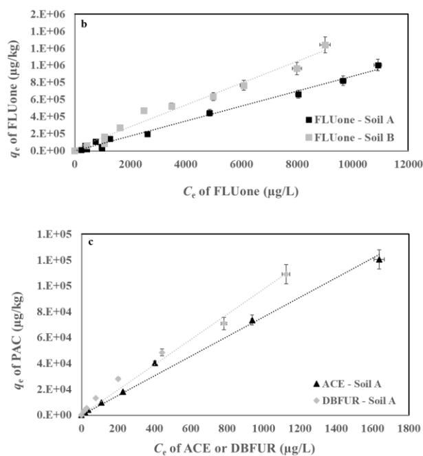
Fig. 2. Sorption isotherms at equilibrium in reference conditions onto soils A and B for FLU (a), FLUone (b) and ACE/DBFUR (c).
