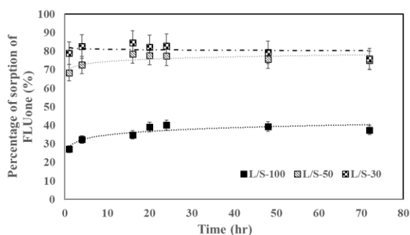
Fig. 3. Sorption kinetics FLUone onto soil A at different L/S ratio. For all L/S values: C_{\text{FLUone}}(0) = 10,000 \mu\text{g/L} .
