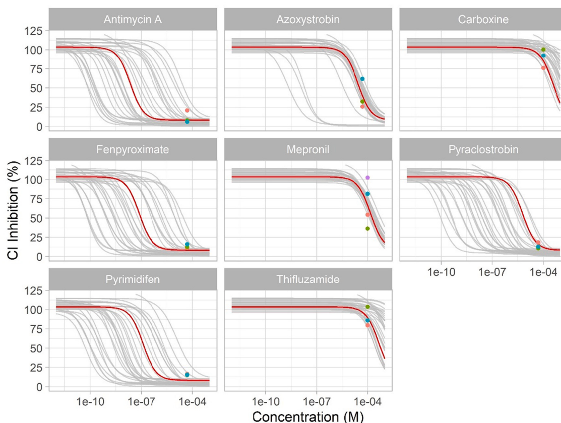
Fig. 8. Modelled dose-responses of complex I inhibition for each validation chemical, when ( y_{minCI} , y_{maxCI} , k_{CI} ) are set to the rotenone values. Red line uses the chemical-specific EC_{50CI} MPV and other qAOP parameters set to the rotenone MPV. Grey lines: 30 samples from the posterior distribution of chemical-specific EC_{50CI} each combined with one sample from the posterior distribution of the other qAOP parameters calibrated on rotenone. (For interpretation of the references to colour in this figure legend, the reader is referred to the web version of this article.)
