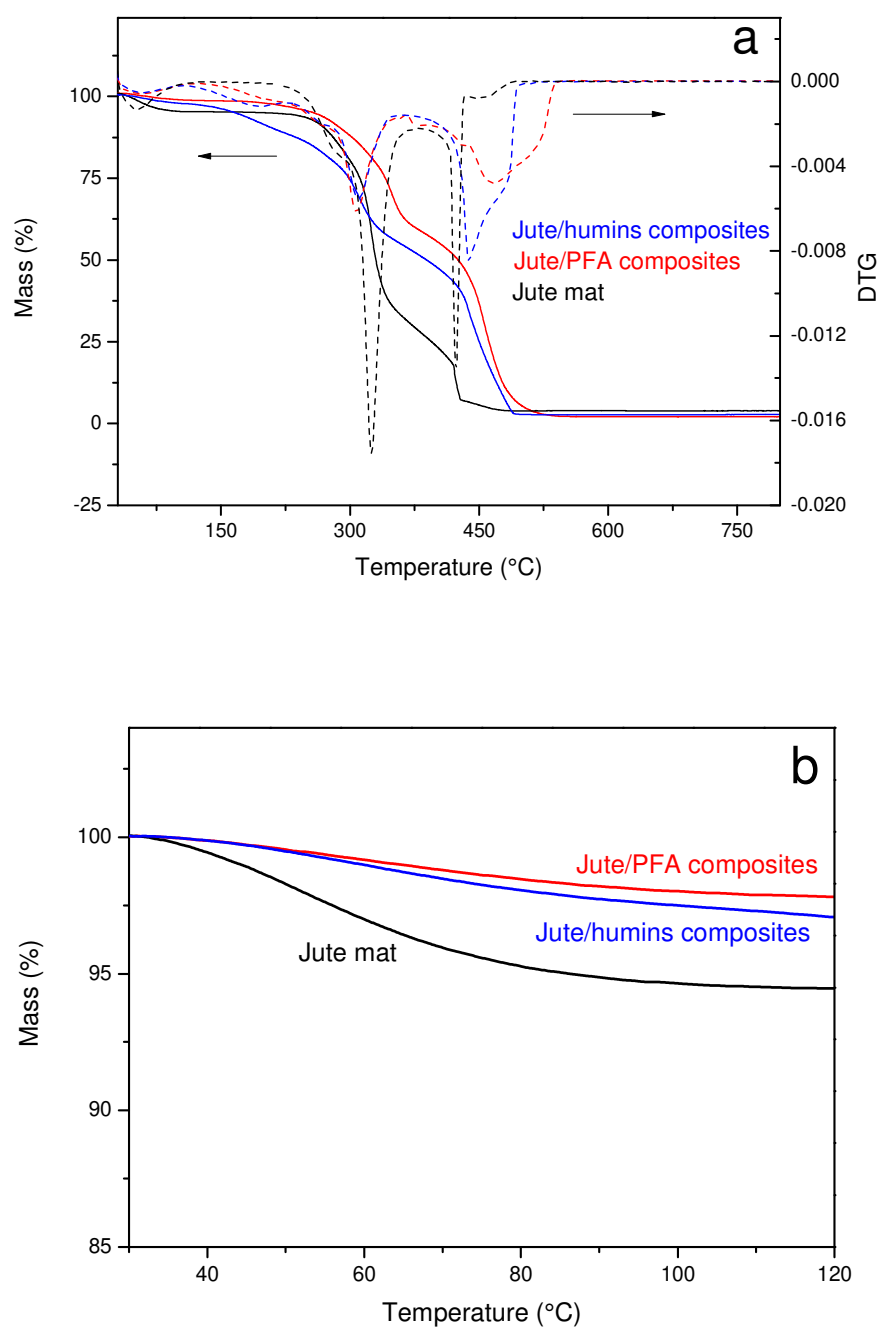
Figure 3a. TG and DTG curves of Jute/PFA and Jute/Humins composites. Neat Jute is given as reference. 3b. Zoom of TG curves of Jute/PFA and Jute/Humins composites in the low temperature region. Neat Jute is given as reference.
