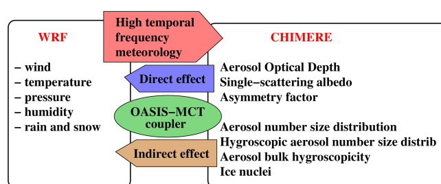
Figure 7. Main principle of the coupling between WRF and CHIMERE for the calculation of the direct and indirect effects of aerosols on meteorology.
