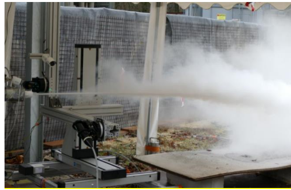
Fig. 9. Test 8b - Rainout evidence. IR screenshot (left), visible (right).
