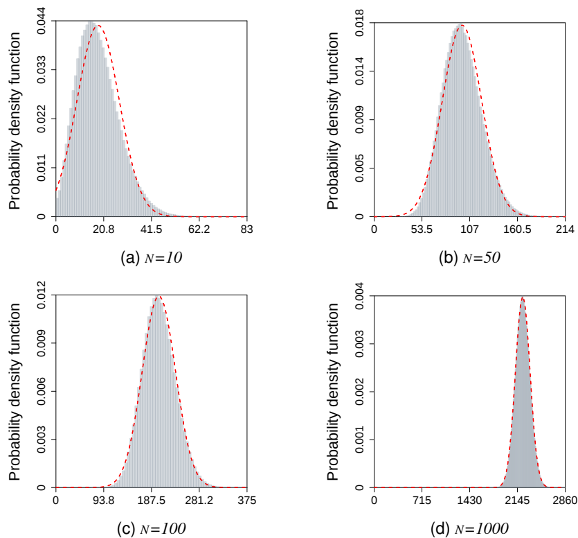
FIGURE 2: Monte-Carlo histograms and probability density functions of the normal approximations. Examples for the sum of 10, 50, 100 and 1000 independent rectified Gaussian variables with mean and standard deviations of their related Gaussian variables uniformly sampled in [-3, 3] and [0, 10]
