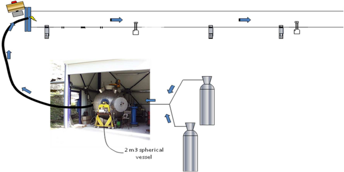
Figure 1 : Overall device
