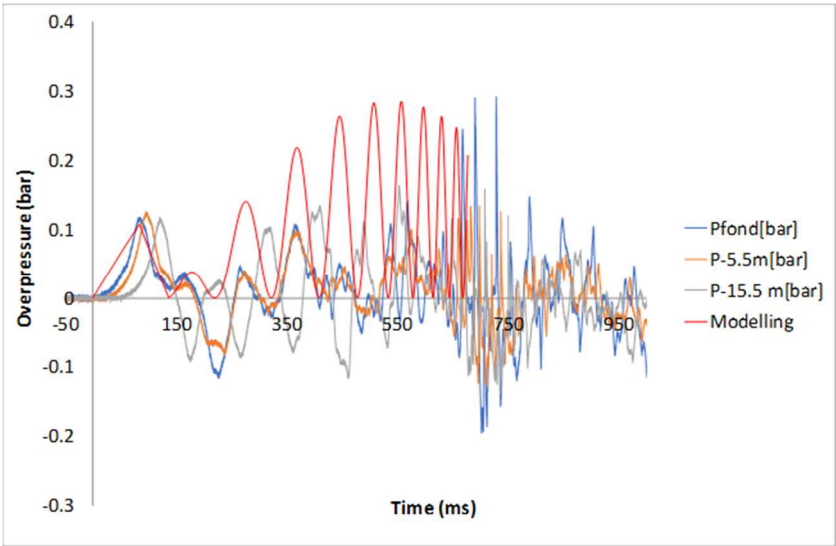
Figure 21 : Estimation of overpressure thanks to the flame velocity
