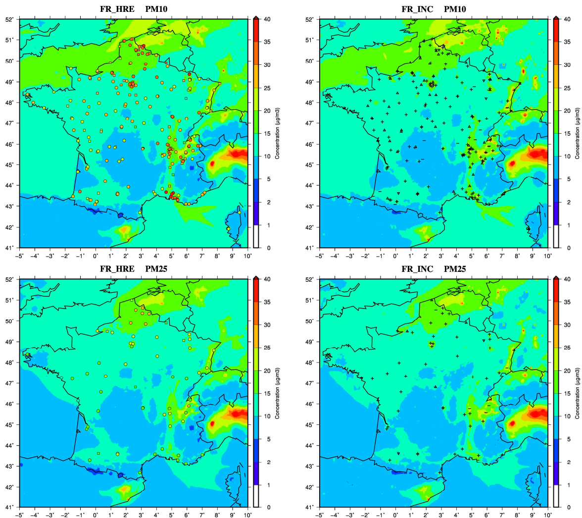
Figure 3: Maps of mean PM10 and PM2.5 concentrations over the 1 st January – 30 June 2011 period for the increment methodology FR_INC (right column) and the CHIMERE high resolution simulation FR_HRE (left column). On the left side: circles and squares filled symbol refer to observations respectively for urban and rural sites. On the right side: bold “triangle up” and “plus” symbols are plotted respectively for rural and urban sites when the increment methodology provides a better Root Mean Square Error compared to the CHIMERE high resolution, bold “triangle down” and “minus” symbols are plotted respectively for rural and urban sites when the increment methodology provides a worse Root Mean Square Error compared to the CHIMERE high resolution.
