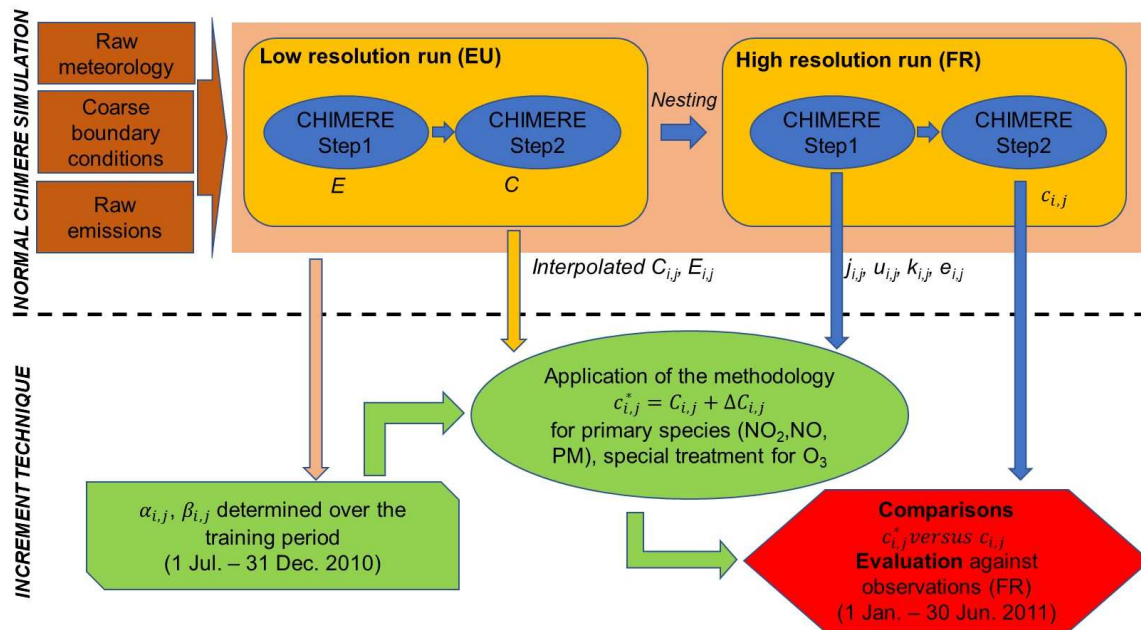
Figure 1: Synoptic scheme of the increment technique compared to the normal CHIMERE simulation over the EU and FR domains. All variables are explained in sections 2.3 and 2.4.
