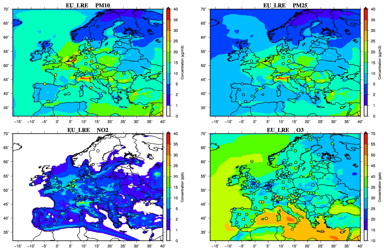
Figure 2 : Maps of mean PM 10 , PM 2.5 , NO 2 and O 3 concentrations over the 1 st January – 30 June 2011 period for the CHIMERE low resolution simulation at the European scale (EU_LRE). Filled circles represent the rural background observation sites issued from the EBAS database.
