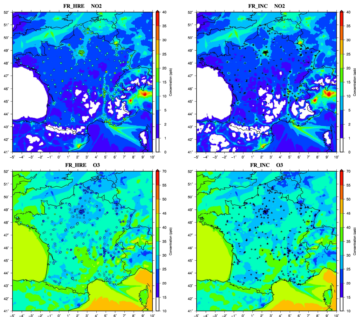
Figure 4: Maps of mean \text{NO}_2 and \text{O}_3 concentrations over the 1 st January – 30 June 2011 period for the increment methodology FR_INC (right column) and the CHIMERE high resolution simulation FR_HRE (left column). On the left side: circles and squares filled symbol refer to observations respectively for urban and rural sites. On the right side: bold “triangle up” and “plus” symbols are plotted when the increment methodology provides a better Root Mean Square Error compared to the CHIMERE high resolution, bold “triangle down” and “minus” symbols are plotted when the increment methodology provides a worse Root Mean Square Error compared to the CHIMERE high resolution.
