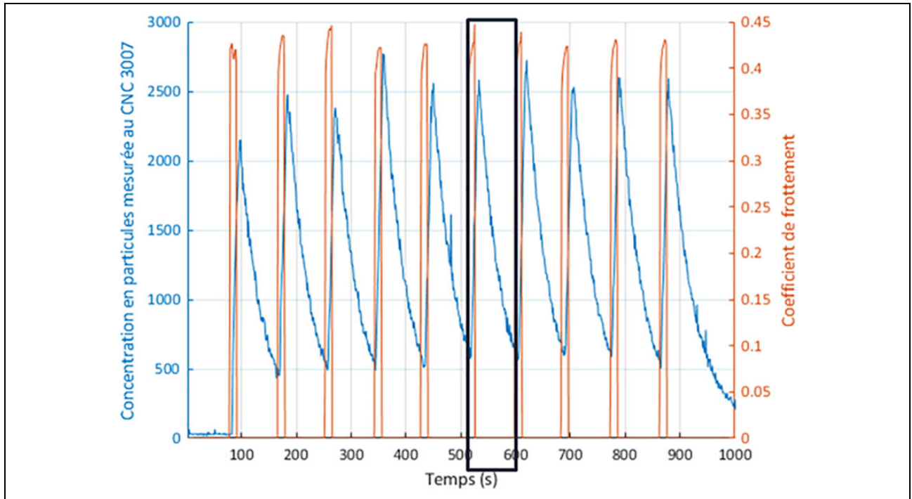
Figure 3. Coefficient of friction and concentration measured by CNC during a test at 1.24 MPa and 25.0 m/s ( PV = 31 \text{ MPa.m/s} ).
