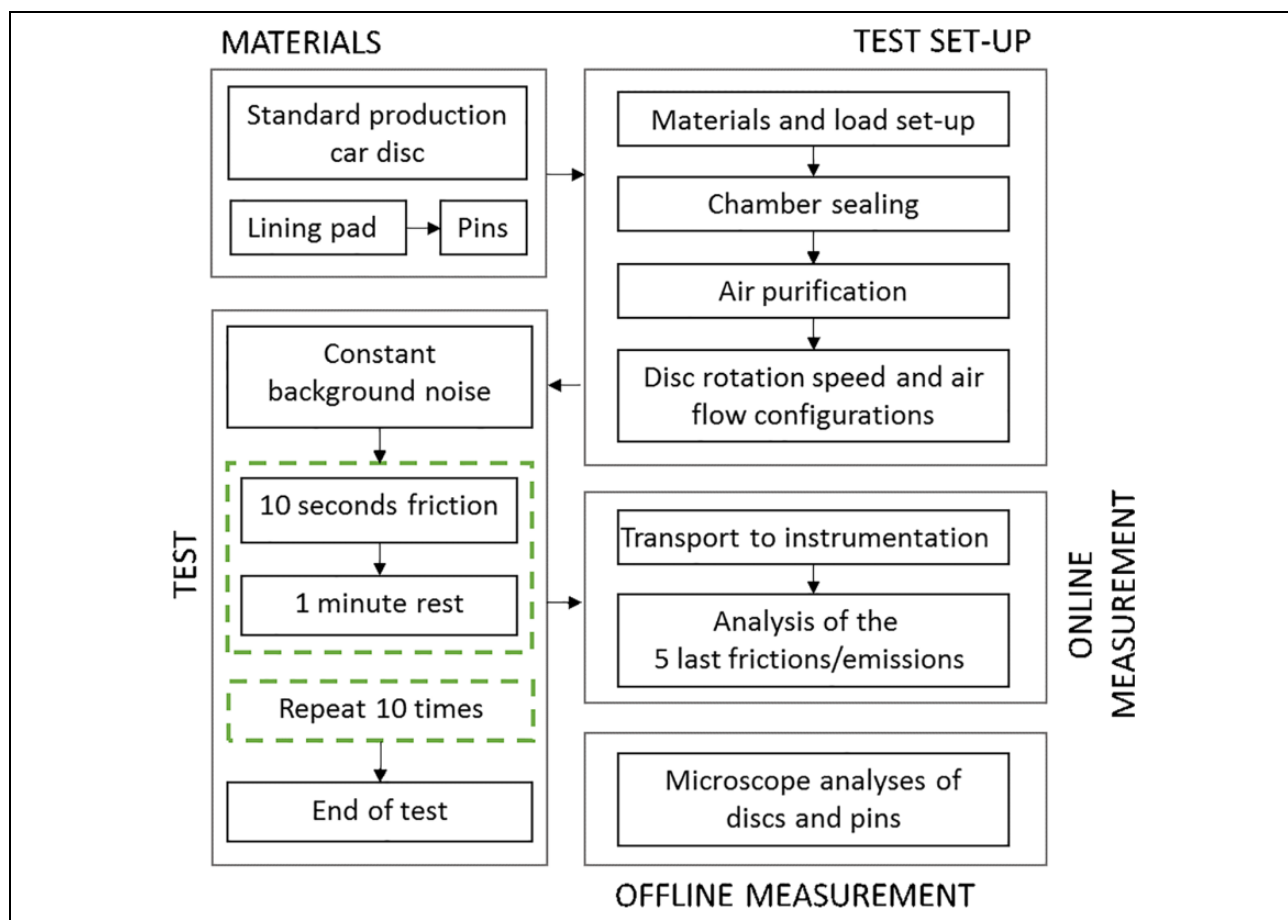
Figure 2. Flow diagram of the testing process.
