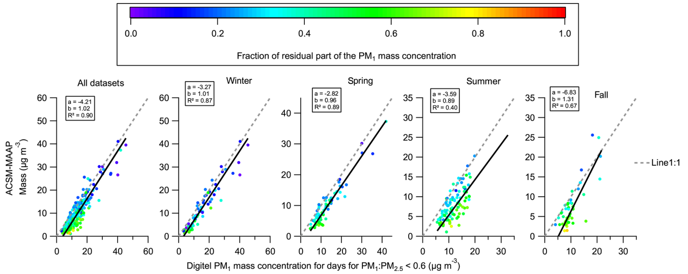
Figure 8. Influence of the residual mass fraction on the PM 1 filter to the mass closure with online ACSM–MAAP-derived mass concentration.
