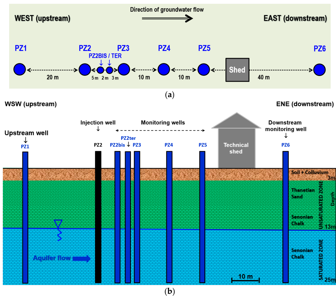
Figure 2. Diagram of the Catenoy experimental site: (a) planimetry; (b) cross-section.
