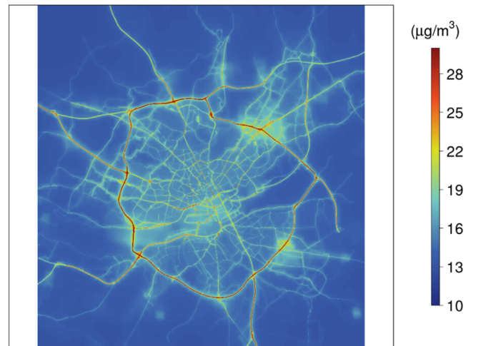
Fig. 6. The annual average of PM 10 concentrations (in µg/m 3 ) for the year 2016 calculated by ADMS-Urban (provided by Air Pays de la Loire) in Nantes and used as the drift in the kriging approach.
