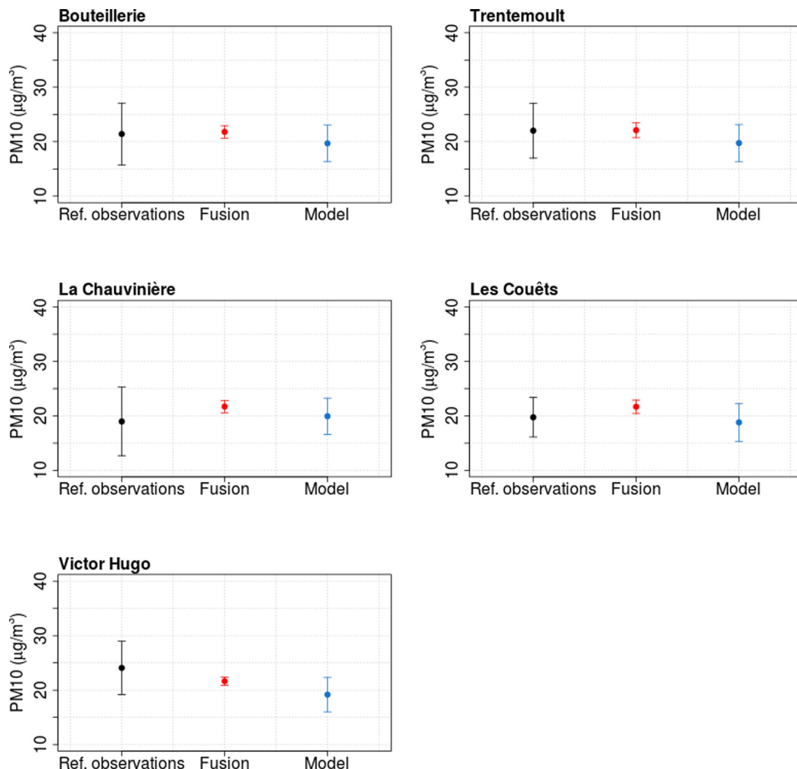
Fig. 11. The daily mean comparison between the PM_{10} observations (in black), the data fusion (in red) and the model (ADMS-Urban, in blue) in \mu\text{g}/\text{m}^3 at each reference station of the Air Pays de la Loire monitoring network on 11/29/2018 in Nantes.
