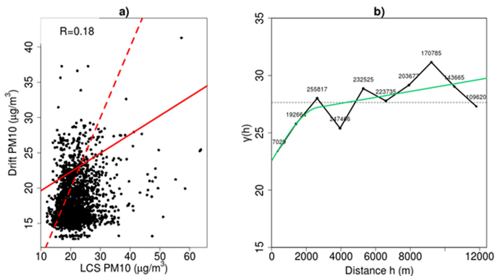
Fig. 8. The correlation plot between the LCS observations and the drift (a) and the variogram of the residuals (b) are derived at 9 am on 11/29/2018. On panel (a), the dashed red line represents x = y and the red solid line corresponds to the estimated regression. On panel (b), the black curve is the experimental variogram and the green curve the estimated variogram model.
