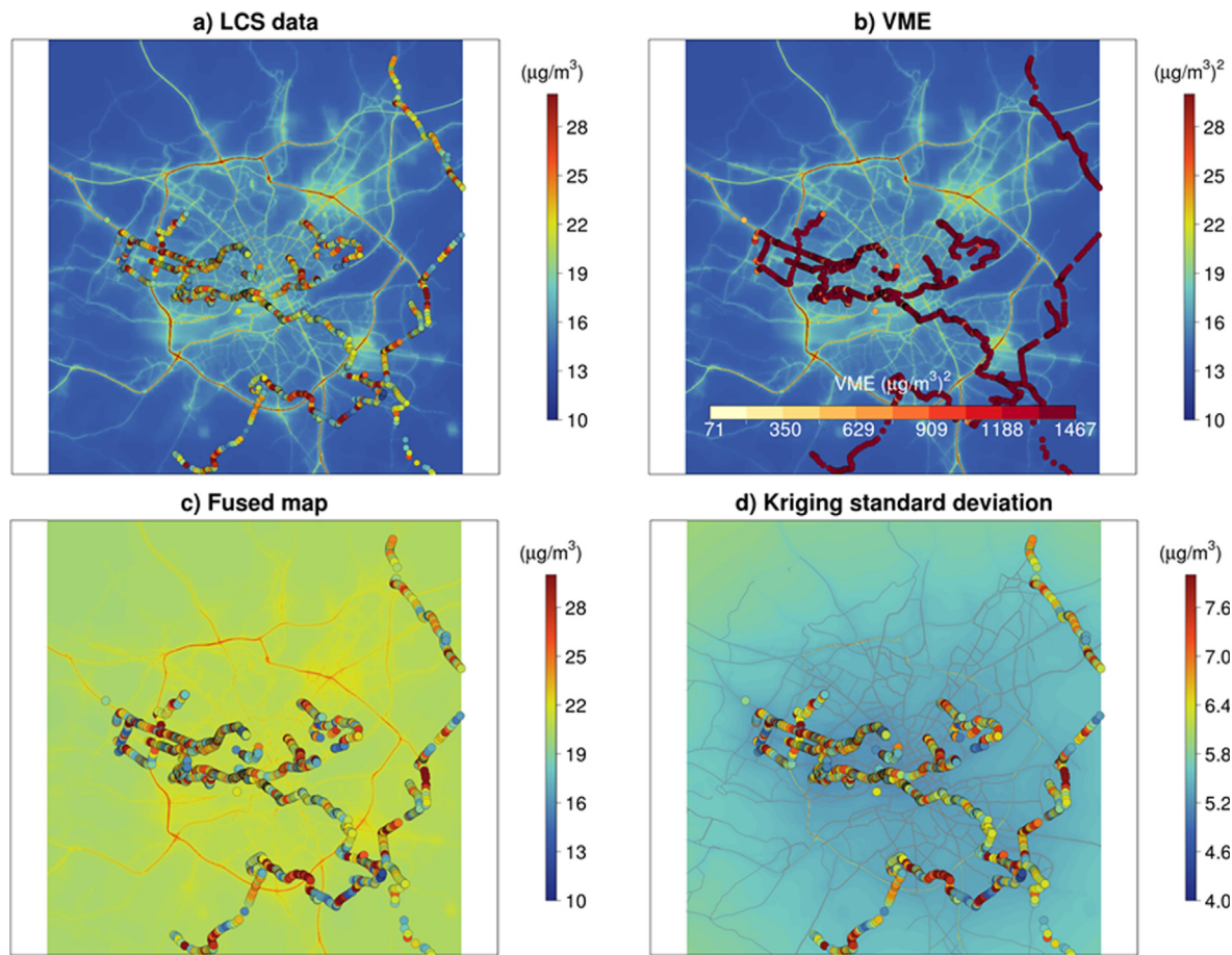
Fig. 7. The PM_{10} LCS observations (in \mu g/m^3 ) overlaid the 2016 annual average of the PM_{10} concentrations (in \mu g/m^3 ) calculated by the ADMS-Urban model that is defined as the drift in the data fusion (a), the variance of the measurement error (VME, in (\mu g/m^3)^2 ) is shown with the drift in the background (b), the hourly fused map with the PM_{10} LCS observations (c) and the kriging standard deviation with the PM_{10} LCS observations and the shapefile of the main roads on the background (d), are presented on 11/29/2018 at 9 am in Nantes.
