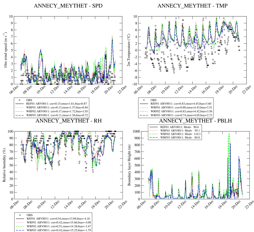
Figure 12. Impact of WRF settings on some meteorological variables at \frac{1}{40}^{\circ} resolution (ARV0011) for the EPII period.
