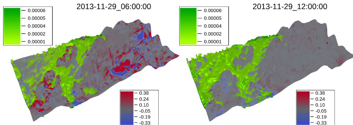
Figure 7. Impact of the on-line coupling on meteorological variables at \frac{1}{10}^\circ resolution (GRE0011) on 29 November at 06:00 UTC (left) 12:00 UTC (right). Color palettes represent the difference between CPL01 and REF01 simulations (green for the cloud water content in \text{kg kg}^{-1} , blue to red the 2 m temperature in ^\circ\text{C} ). Imagery produced by VAPOR ( www.vapor.ucar.edu ), a product of the Computational Information Systems Laboratory at the National Center for Atmospheric Research [71].
