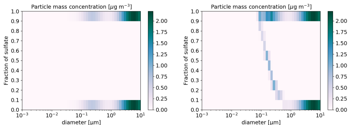
Figure 8. Particle mass concentration ( \mu\text{g m}^{-3} ) for the condensation test case, as a function of size and composition: initial concentrations (left) and after 12 h of simulation (right).
