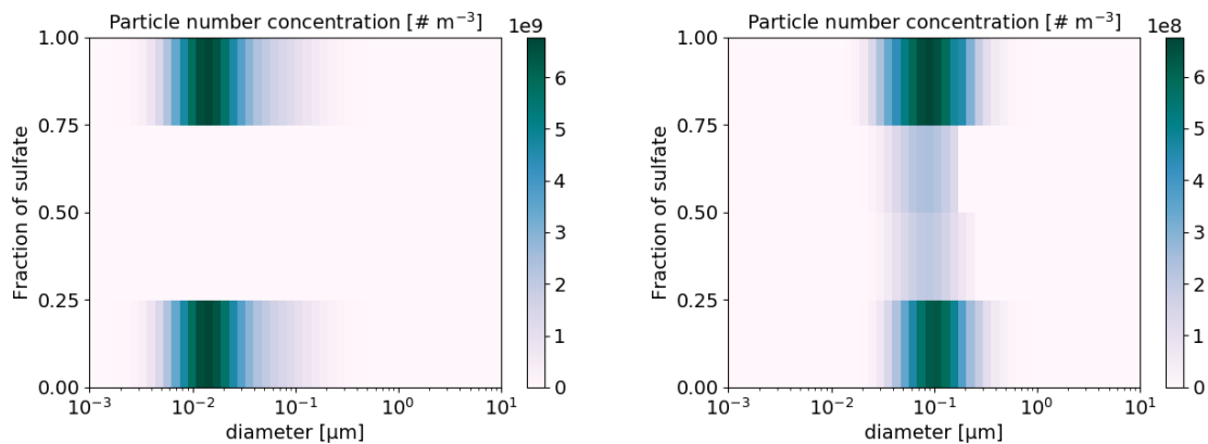
Figure 7. Particle number concentration ( \# m^{-3} ) for the coagulation test case, as a function of size and composition: initial concentrations (left) and after 12 h of simulation (right).
