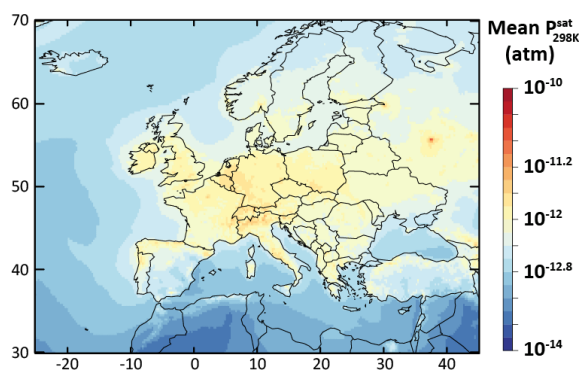
Figure 10. Simulated average volatility of OA in term of P_{298\text{K}}^{\text{sat}} upon Europe during the July–August 2013 period for the ref-VBS-GECKO model configuration.
