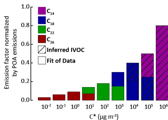
Figure 11. Distribution of the VBS-GECKO species into the S/IVOC volatility bins by Robinson et al. (2007). Normalized emission factors by POA emissions for IVOCs are used for the IVOC_{150POA} model configuration.
