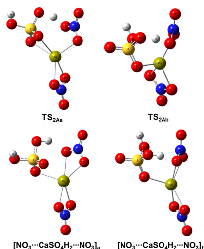
Figure 3. Transition states and complexes of the reactions of HNO 3 and CaSO 4 .
