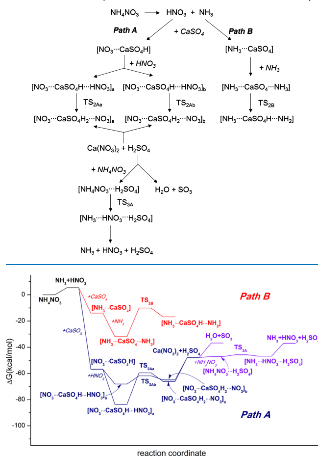
Figure 2. Gibbs free-energy profile for the reaction between AN and CaSO 4 .
