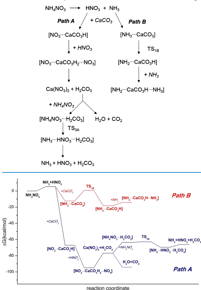
Figure 1. Gibbs free-energy profile for the reaction between AN and CaCO 3 .
