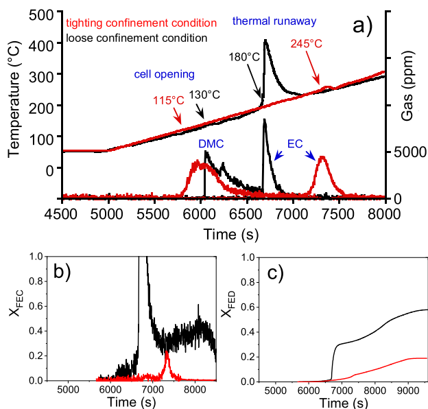
Figure 3. (a) Prototype cells surface temperature and production of dimethyl carbonate (DMC) and ethylene carbonate (EC) solvents detected from FTIR analysis as function of time during thermal stability tests. The prototype cells were subjected to a continuous ramp of 5\text{ }^{\circ}\text{C min}^{-1} up to 300\text{ }^{\circ}\text{C} under loose (black lines) and tighting (red lines) confinement conditions. Comparison of the evolution of the (b) fractional effective concentration ( X_{\text{FEC}} ) and (c) fractional effective dose ( X_{\text{FED}} ).
