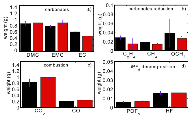
Figure 6. Gas amount emitted during thermal stability tests of prototype cells containing a reference electrolyte with (red) and without (black) 2 wt% VC, under loose confinement condition.
