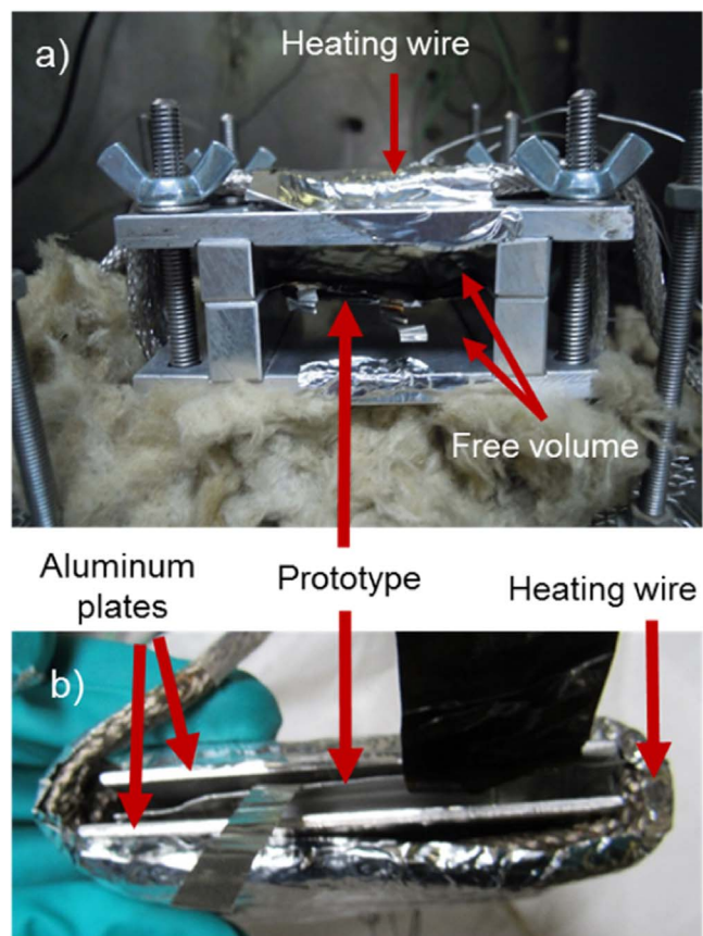
Figure 2. Pictures of holders used for thermal stability tests on prototype pouch cells under (a) loose and (b) tightening confinement conditions.
