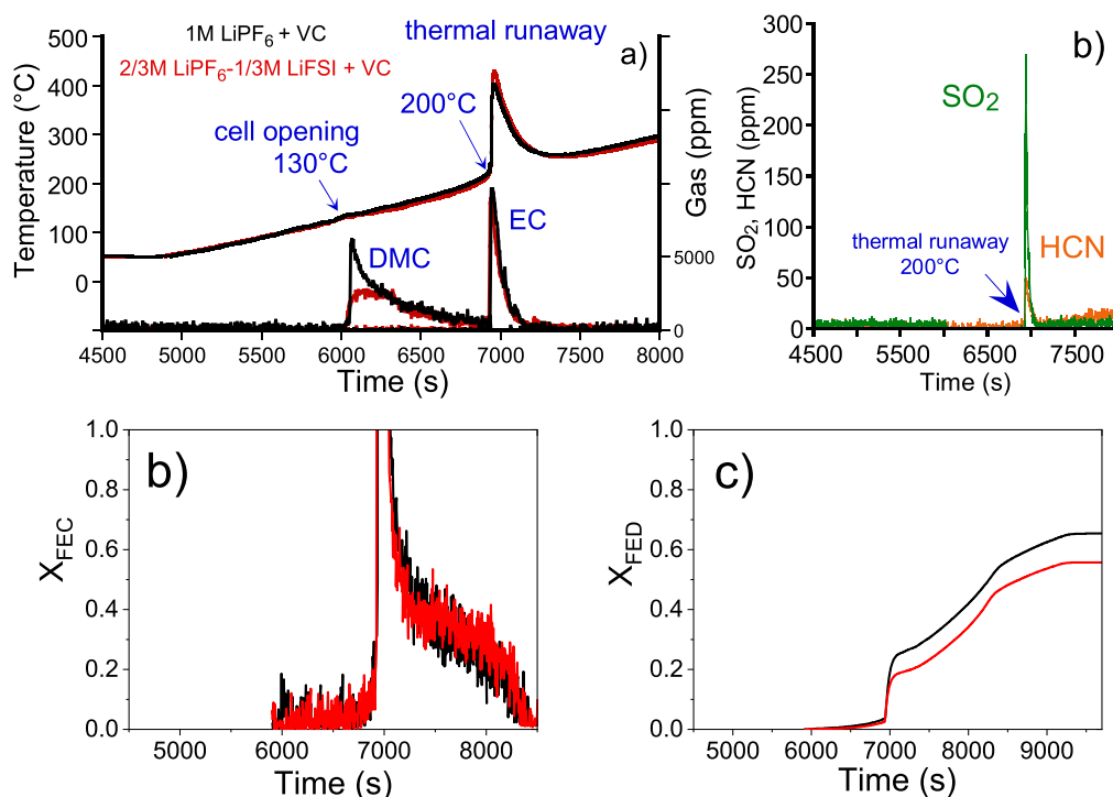
Figure 7. (a) Surface temperature and production of DMC and EC solvents of prototype cells with a reference electrolyte +2 wt% VC (black) and with a 2/3 M LiPF_6 –1/3 M LiFSI + 2 wt% VC electrolyte (red) as function of time during thermal stability tests performed under a continuous ramp of 5 °C min −1 up to 300 °C and a loose confinement condition. (b) Concentration profiles of SO_2 and HCN for the prototype cells containing a 2/3 M LiPF_6 –1/3 M LiFSI + 2 wt% VC electrolyte. Comparison of the evolution of the (c) fractional effective concentration ( X_{FEC} ) and (d) fractional effective dose ( X_{FED} ).
