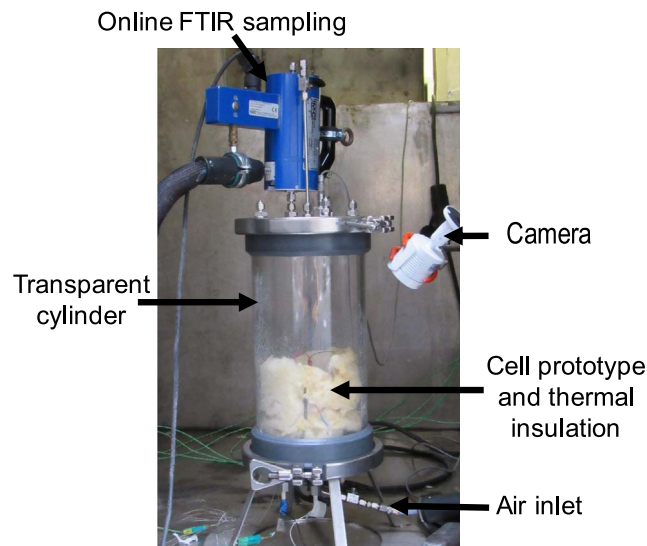
Figure 1. Heating device coupled with a FTIR gas analyzer for thermal stability tests on 0.6 Ah prototype pouch cells.
