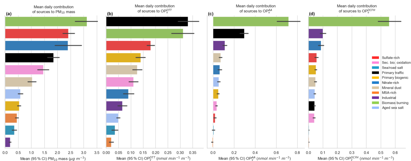
Figure 6. Overall daily mean OP_v contribution of the sources to PM 10 , OP_v^{DTH} , OP_v^{AA} , and OP_v^{DCFH} using MLR analysis in the form of mean and 95 % confidence interval of the mean (error bar) ( n = 378 samples).
