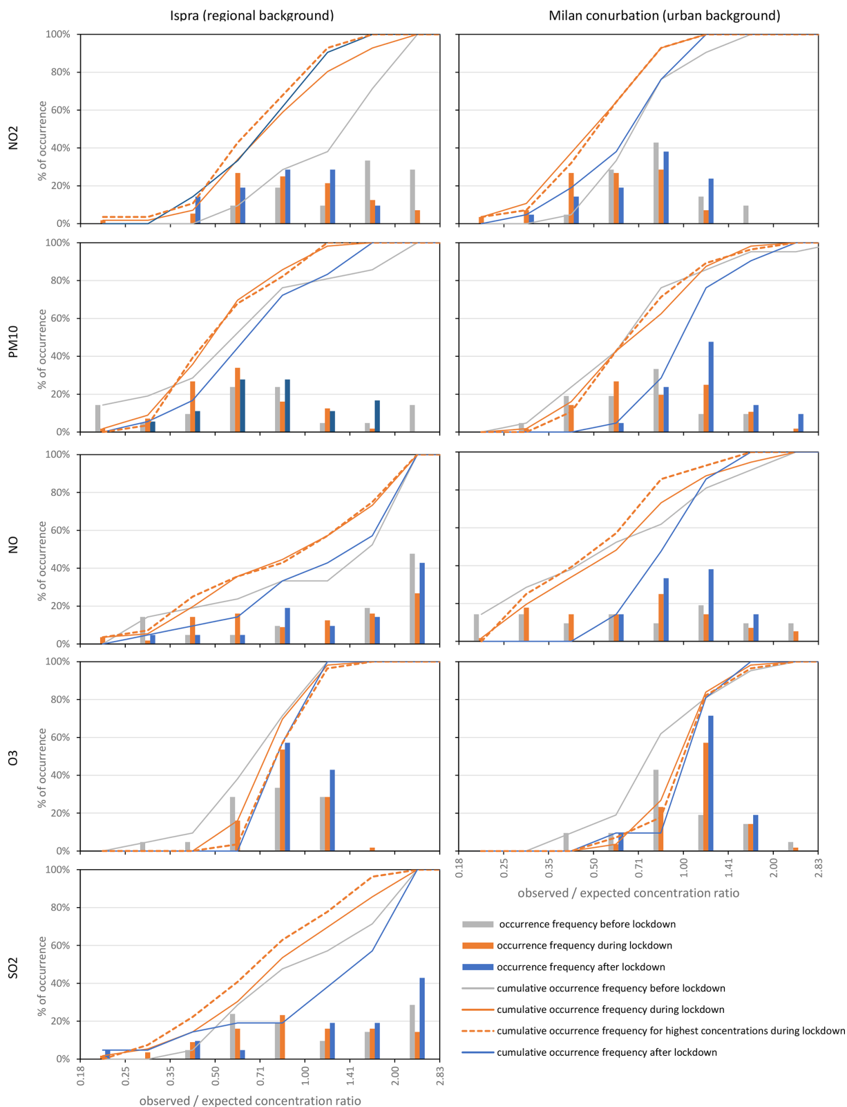
Figure 4. Occurrence frequency distributions of 2020 observed/expected concentration ratios ( \text{Obs}_{2020} / \text{Exp}_{2020} ) for NO 2 , PM 10 , NO, O 3 and SO 2 during the lockdown period and during the 3 weeks before and after the lockdown period in Ispra (left) and the Milan conurbation (right). Lines show cumulative frequencies of occurrence. Dashed lines show the cumulative frequency of occurrence of \text{Obs}_{2020} / \text{Exp}_{2020} ratios for the 28 d corresponding to the highest CAMS forecast values. Note: the last bin for NO in Ispra contains all values >2.
