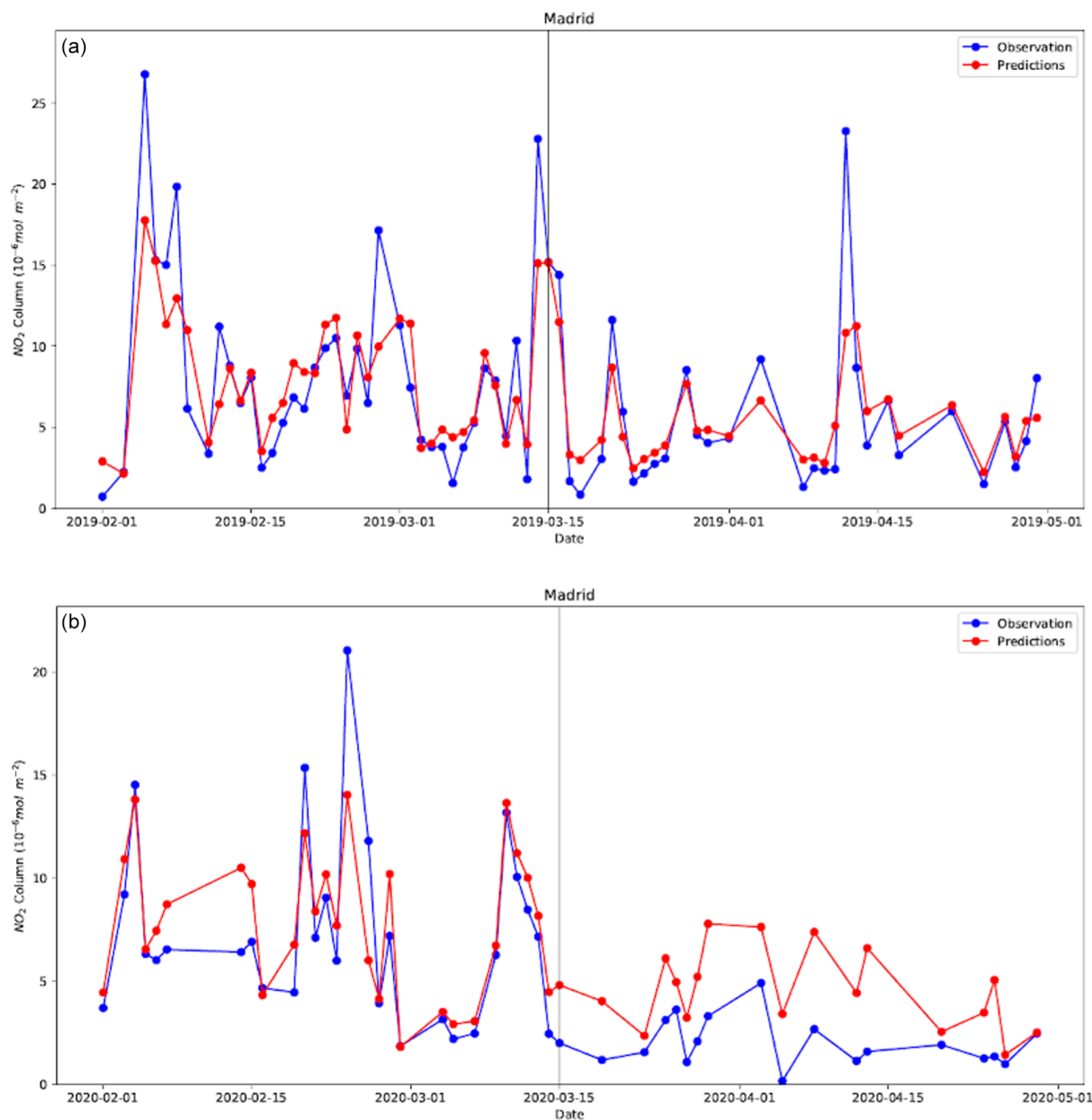
Figure 5. Example of a time series over Madrid illustrating the performance of the machine learning NO 2 column predictions for February–March–April 2019 (a) and the same period in 2020 (b).
