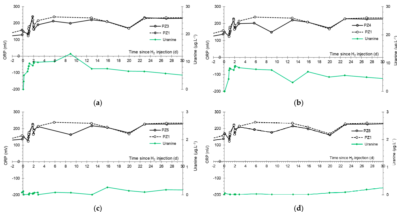
Figure 16. Comparative evolution of the oxidation-reduction potential and the tracer concentration at the other downstream piezometers: (a) PZ3 (10 m); (b) PZ4 (20 m); (c) PZ5 (30 m); and (d) PZ6 (60 m).
