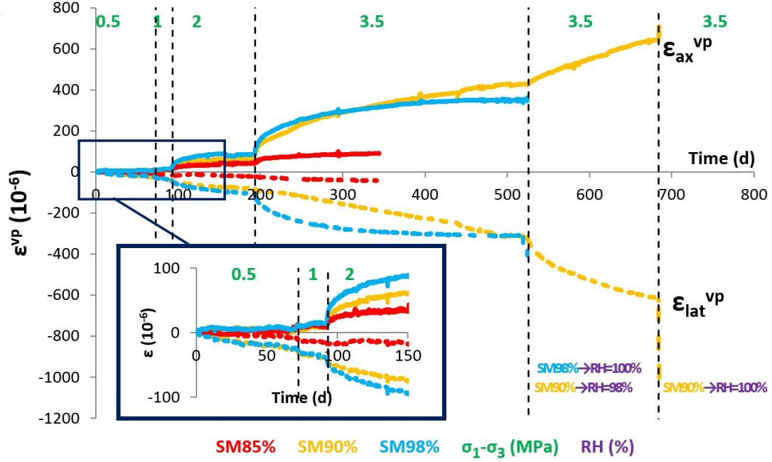
Figure 4. Creep curves of Saint-Martin-le-Noeud underground chalk mine. Axial ( \epsilon_{ax}^{vp} ) and lateral ( \epsilon_{lat}^{vp} ) strains as a function of time.
