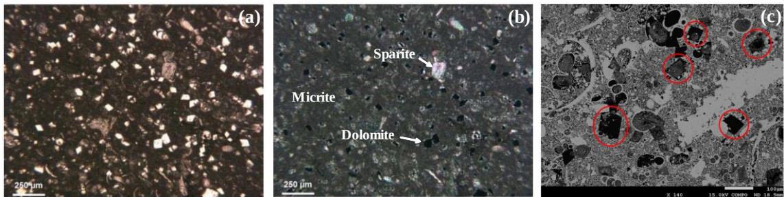
Figure 3. Microscopic analysis: (a) natural light; (b) polarized light; (c) SEM image.
