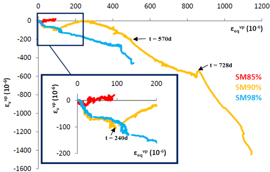
Figure 6. Creep curves of Saint-Martin-le-Noeud underground chalk mine. Viscoplastic dilatancy ( \varepsilon_v^{vp} ) versus deviatoric viscoplastic strain ( \varepsilon_{eq}^{vp} ).
