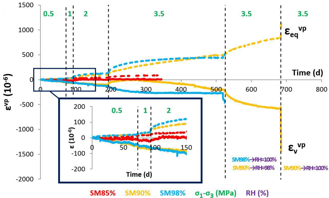
Figure 5. Creep curves of Saint-Martin-le-Noeud underground chalk mine. Volumetric ( \epsilon_v^{vp} ) and deviatoric ( \epsilon_{eq}^{vp} ) strains as a function of time.
