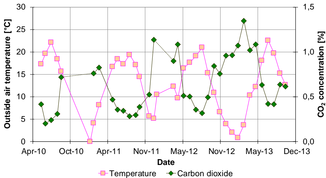
Figure 4. Influence of the natural thermal draught on CO 2 concentration in a fracture at surface in the “Cité Belle Roche”.
