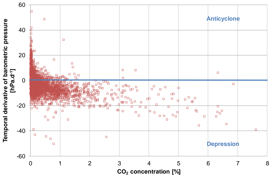
Figure 3. Temporal derivative of the barometric pressure versus the CO 2 concentration in a fracture at surface in the “Cité Belle Roche”.
