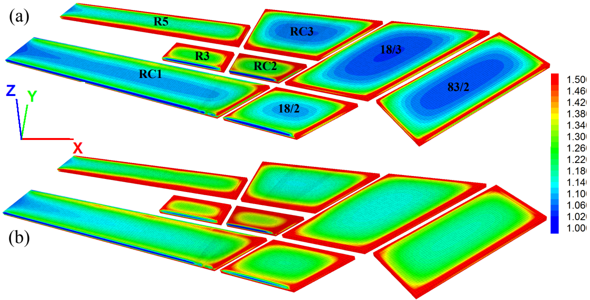
Fig. 5. Normalized vertical stress distribution ( \sigma_{zz}/\sigma_{zz(ini)} ) (a) after excavation of shaft station galleries (b) after panels excavation in 1993.
