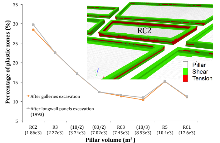
Fig. 6. Shear and tension plastic volume (%) on shaft station pillars.
