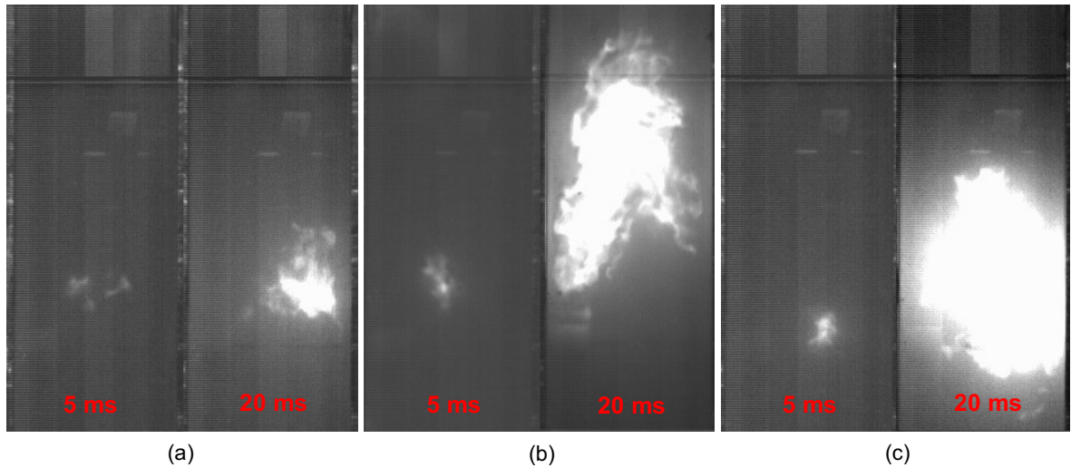
Figure 5: Visualization of flame propagation of nanocellulose at 5 ms and 20 ms for ignition delay times of (a) 60 ms (b) 130 ms (c) 180 ms.
