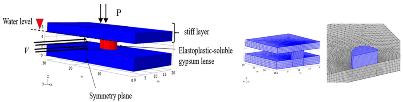
Figure 29. Gypsum pillar model and boundary conditions (left), mesh and zoom (right)
