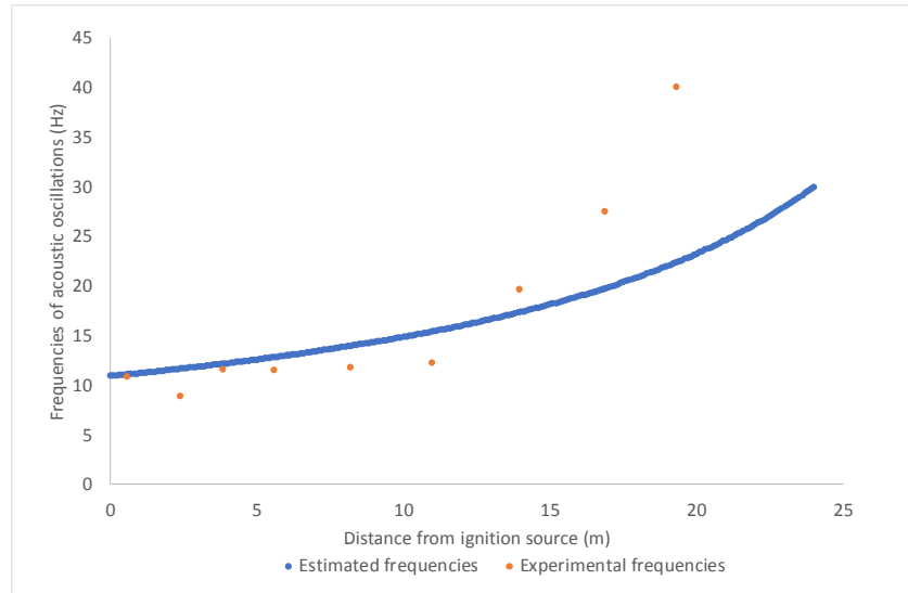
Figure 19 : Comparison between the estimated frequencies and the frequencies deduced from the flame velocity
