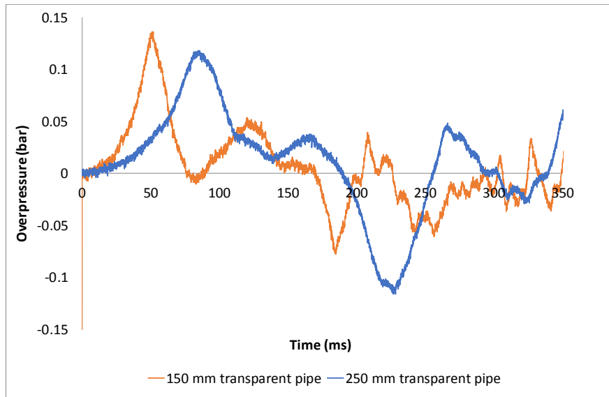
Figure 14: Impact of the tube diameter in the 24 m long transparent tube with diameters of 150 and 250 mm for stoichiometric methane/air mixture
