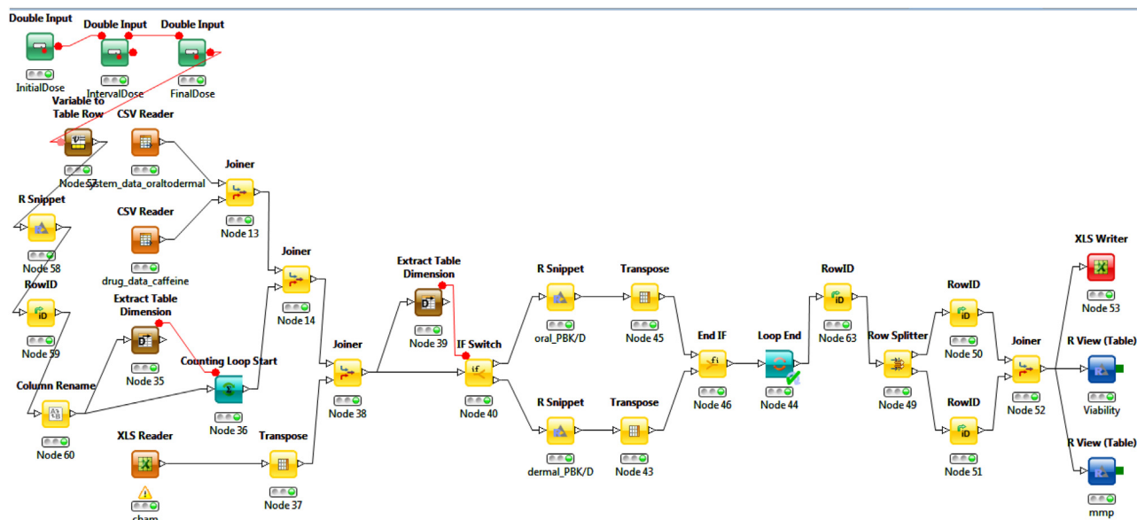
Fig. 9. Schematic representation of a KNIME work-flow developed for PBPK modeling for caffeine effects after oral and dermal exposure. The work flow automatizes data input, model parameters' setting, simulation calls and output to different data streams. The core calculation are done in the "R snippet" nodes in the middle.
