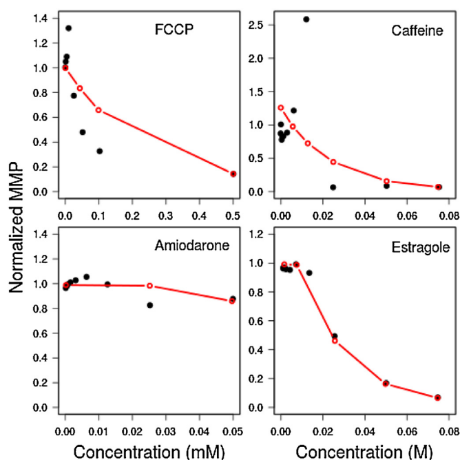
Fig. 1. Observed (black dots) and VCBA model simulated values (red circles and lines) of mitochondrial membrane potential in HepaRG cells exposed in vitro to four test compounds; carbonyl cyanide- p -trifluoromethoxyphenylhydrazone (FCCP), caffeine, amiodarone, and estragole. (For interpretation of the references to colour in this figure legend, the reader is referred to the web version of this article.)
