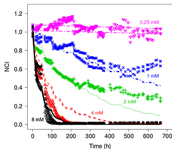
Fig. 3. Normalized Cell Index (NCI) of HepaRG cells exposed every 2–3 days to coumarin at various concentrations for 4 weeks. The data and the model predictions are represented by points and lines, respectively.
