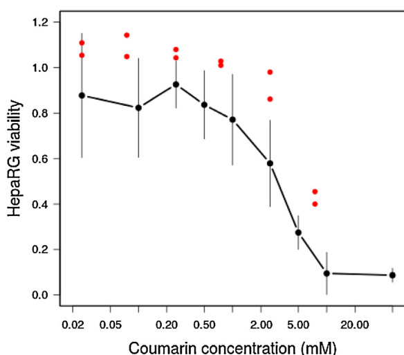
Fig. 4. Comparison of HepaRG cell viability exposed to coumarin at 24 h, as measured by Cellomics and estimated by the VCBA model (black dots) or impedance measurements and Teng's model (red dots). (For interpretation of the references to colour in this figure legend, the reader is referred to the web version of this article.)
