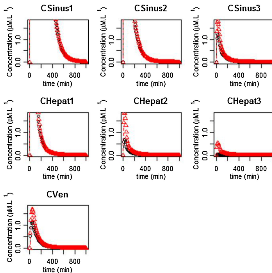
Fig. 7. Model prediction of acetaminophen concentration-time profiles in three zones (1: periportal; 2: midlobular; 3: pericentral) of the liver sinusoid vessels or hepatocytes, and in venous blood, with zonation of metabolism (red curves) or without zonation (black curves), after a 5 mg/kg oral administration of acetaminophen of an adult man. The transport rate to hepatocytes was 1.40 \times 10^{-1} \text{ L/min} , and 1.08 \times 10^{-2} \text{ L/min} along the sinusoids. (For interpretation of the references to colour in this figure legend, the reader is referred to the web version of this article.)
