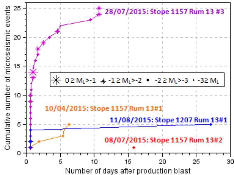
Figure 4 Microseismic events detected and located in a 25 m-radius around each production blast over the corresponding post-blast periods. The size of the stars is proportional to the estimated M_L of the events, varying between -3 and 0. The plot colors correspond to the colors of the stopes as identified in Fig. 1
