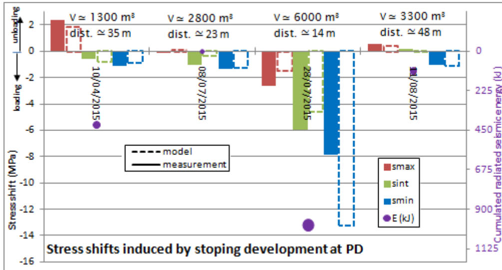
Figure 6 Measured and modeled stress shifts (smax = major, sint = intermediary, smin = minor) induced by stoping development at PD between April and August 2015. Information on the excavated volume (V), the distance from the cells (dist.) and the cumulated radiated seismic energy (purple circle) are added
