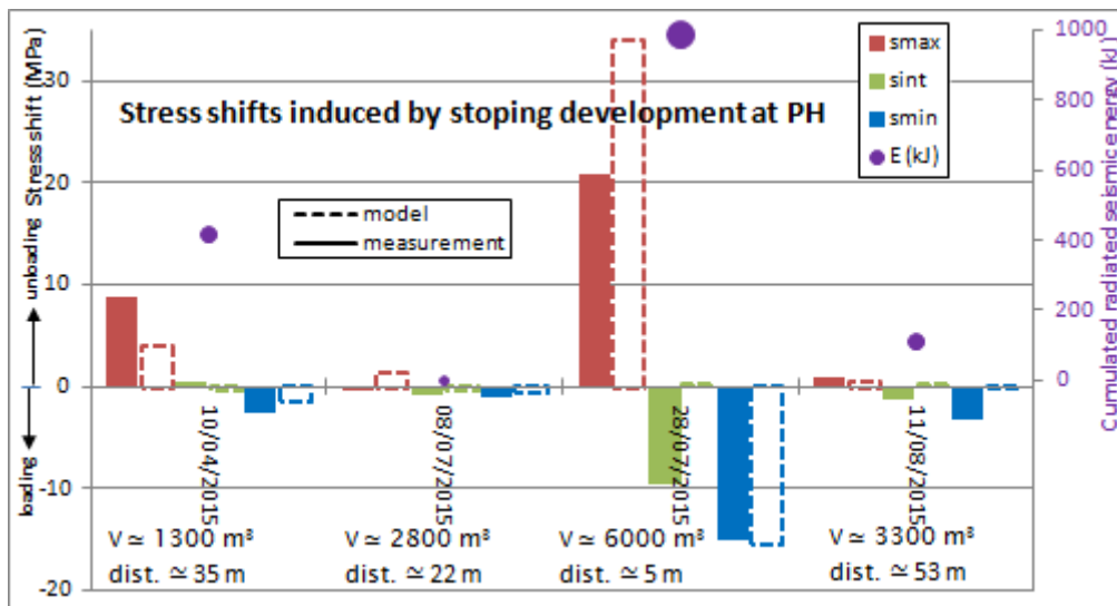
Figure 5 Measured and modeled stress shifts (smax = major, sint = intermediate, smin = minor) induced by stoping development at PH between April and August 2015. Information on the excavated volume (V), the distance from the cells (dist.) and the cumulated radiated seismic energy (purple circle) are added
