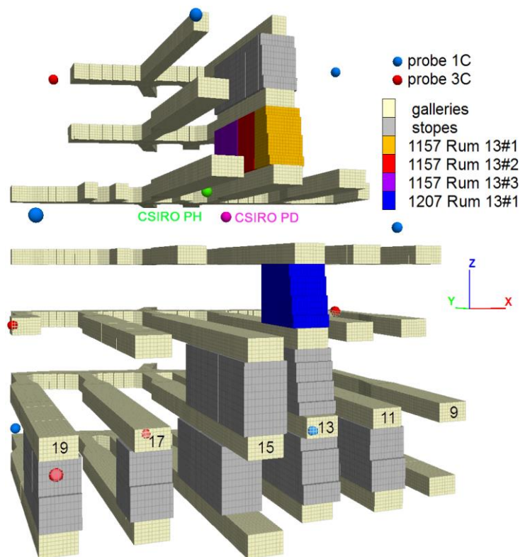
Figure 1 3D view of Lappberget monitored section with successive stope production in yellow, red, purple and blue for the 4 stress shifts that are analyzed in the present study and in grey for the other productions. CSIRO cells and microseismic 1C and 3C probes are also indicated as well as the primary stopes number (from 9 to 19)
