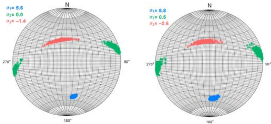
Figure 3 Stress shift assessments (in MPa) calculated with the strain shift recorded at the stress monitoring CSIRO HI cell PH after blast 1157 13#1 (10/04/2015). Left: shift between states immediately before and after the blast; right: shift between states immediately before the blast and 10 days after the blast. The indicated North corresponds to the predefined North of the mine (along Y axis on Fig. 1)
