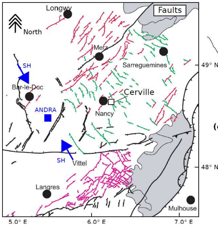
(a) Regional tectonic map after Andre (2003)
