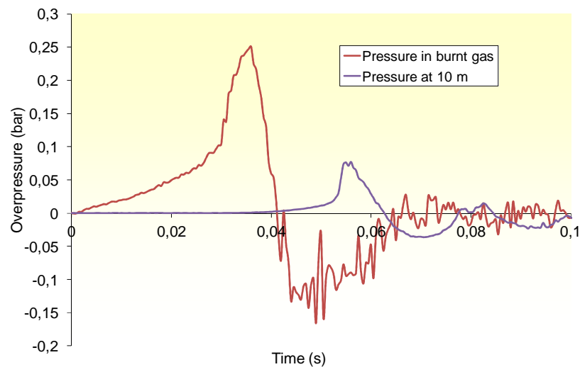
Figure 11. Burnt gas overpressure and overpressure at 10 m – Quiescent mixture (mixture 1 : 40 % H 2 , 20 % O 2 , 40 % N 2 )
