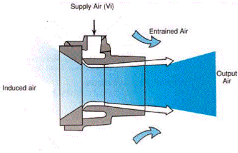
Figure 4. Principle of jetflow
