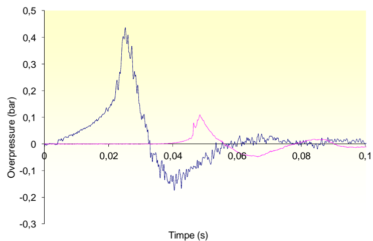
Figure 13. Burnt gas overpressure and overpressure at 10 m – Quiescent mixture (mixture 2 : 45 % H 2 , 22.5 % O 2 , 32.5 % N 2 )
