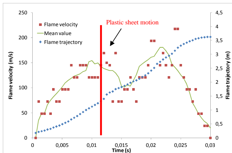
Figure 15. Flame trajectory and flame propagation velocity – Mixture 1
