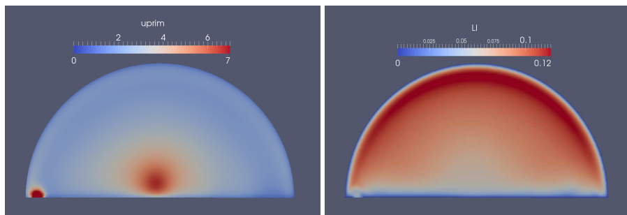
Figure 9. PIMPLEFOAM simulation for fan configuration – u' and L_t
