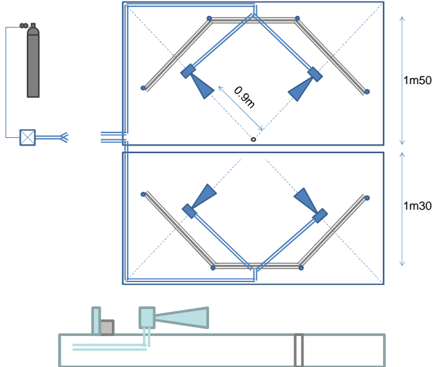
Figure 5. Gas dispersion device
