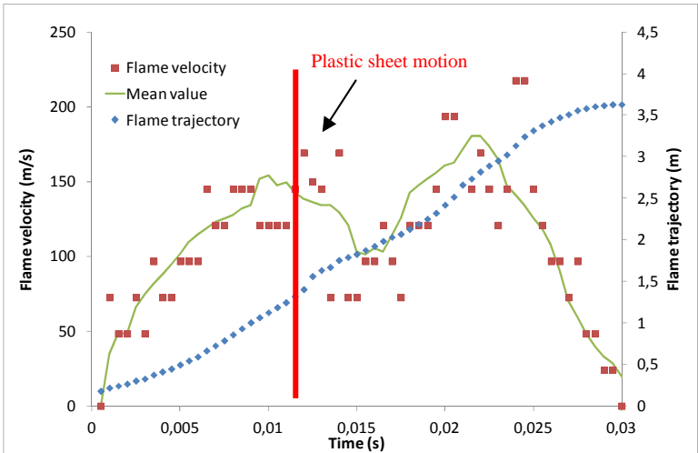
Figure 15. Flame trajectory and flame propagation velocity – Mixture 1
