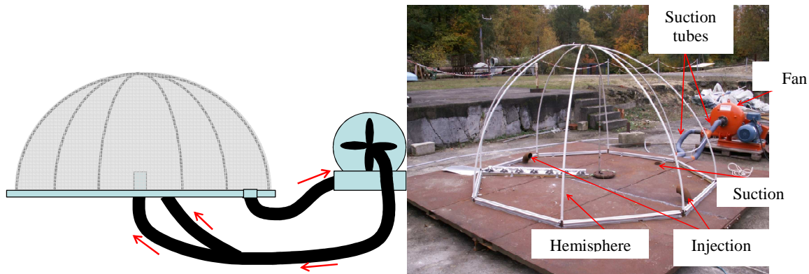
Figure 7. Earlier version of the test platform
