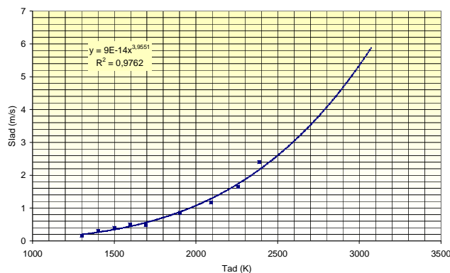
Figure 6. Laminar flame speed vs adiabatic combustion temperature for stoichiometric H2-O2 mixture diluted with N2
