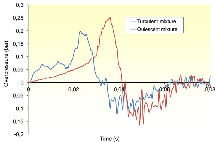
Figure 16. Burnt gas overpressures for the quiescent and the turbulent mixtures
