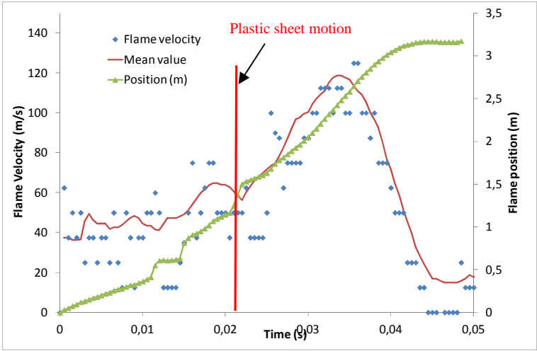
Figure 14. Flame trajectory and flame propagation velocity – Mixture 1
