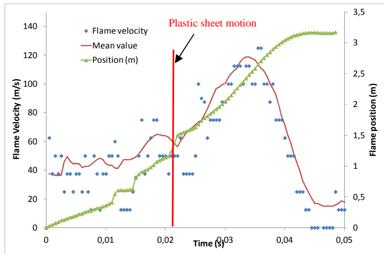
Figure 14. Flame trajectory and flame propagation velocity – Mixture 1
