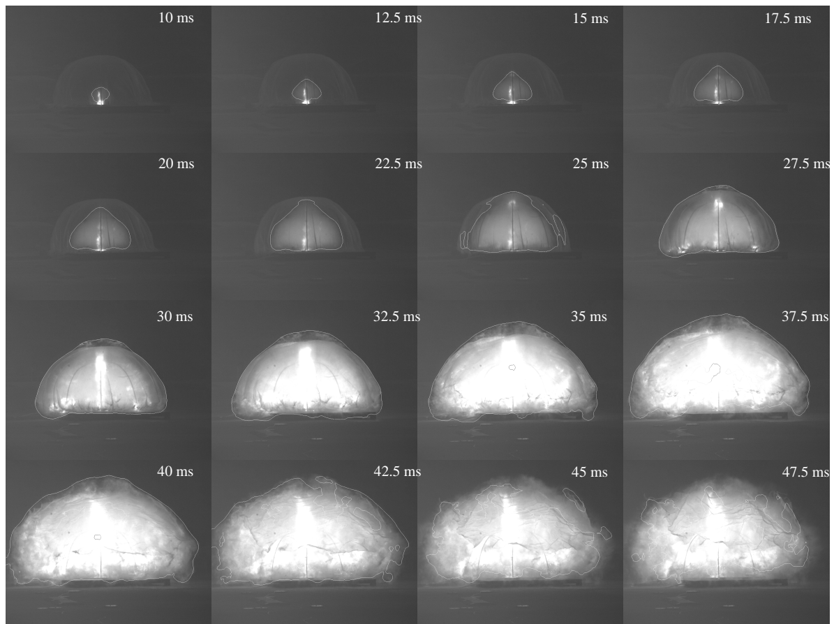
Figure 12. Evolution of the flame at different times - The time between two pictures is 2.5 ms
