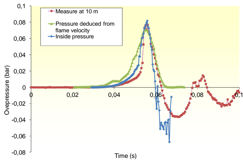
Figure 18. Reconstitution of 10 m pressure signal from flame velocity and inside overpressure
