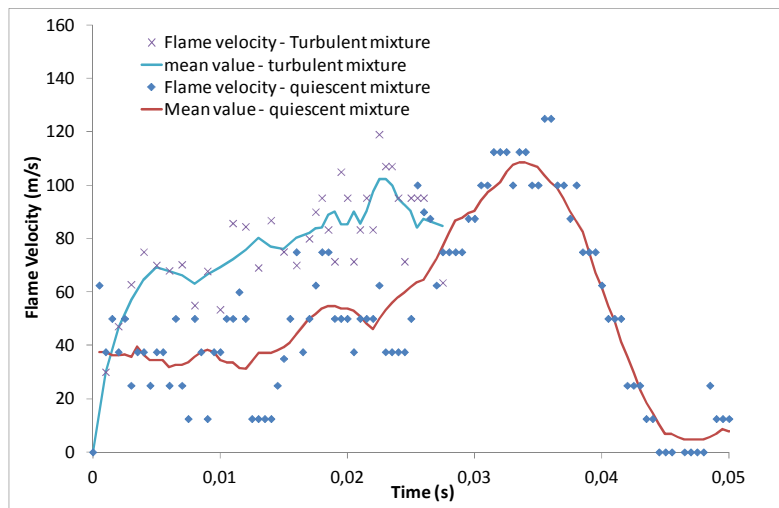
Figure 17. Flame velocities for the quiescent and the turbulent mixtures
