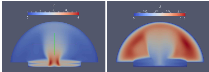
Figure 10. PIMPLEFOAM simulation for jetflow configuration – u' and L_t
