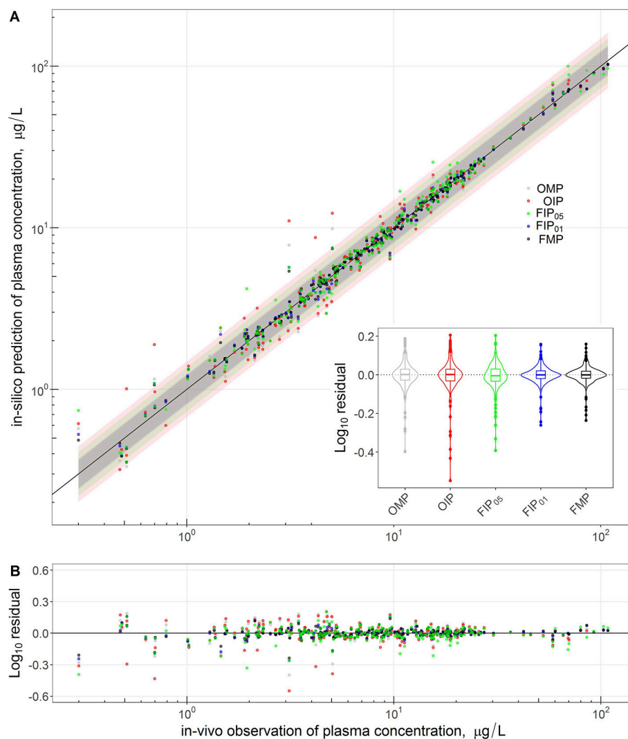
FIGURE 4 | Comparison and global evaluation of the PBPK simulation results with residual properties estimation to determine the accuracy (residual median) and the precision (residual distribution) in model performance. The top (A) shows the relationships between experimental data (x-axis) and PBPK model predictions (y-axis) and 95% predicted interval for five model parameter settings. The bottom (B) shows the residuals from the predicted and experimental values to evaluate the accuracy and precision of model performance.
