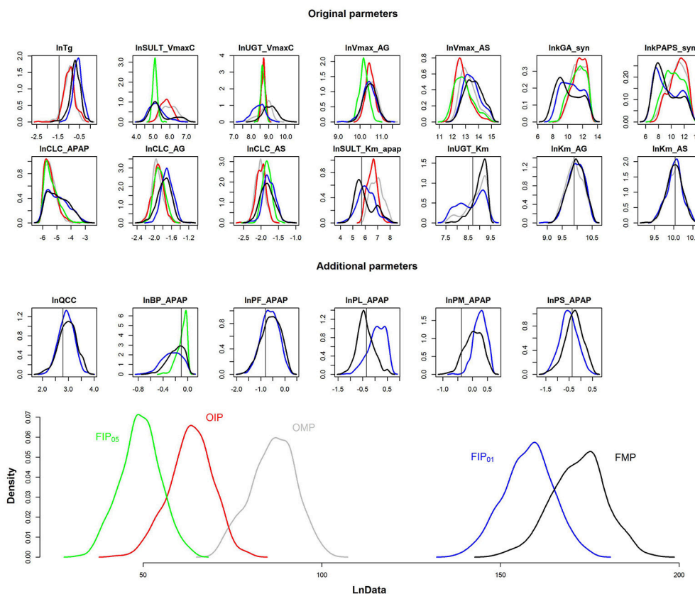
FIGURE 6 | Comparison of the marginal posterior distributions of influential parameters and log-likelihood (LnData) for OMP (gray), OIP (red), FMP (black), FIP 05 (green), FIP 01 (blue). The vertical line represents the prior mean and nominal value of original and additional parameters, respectively.
