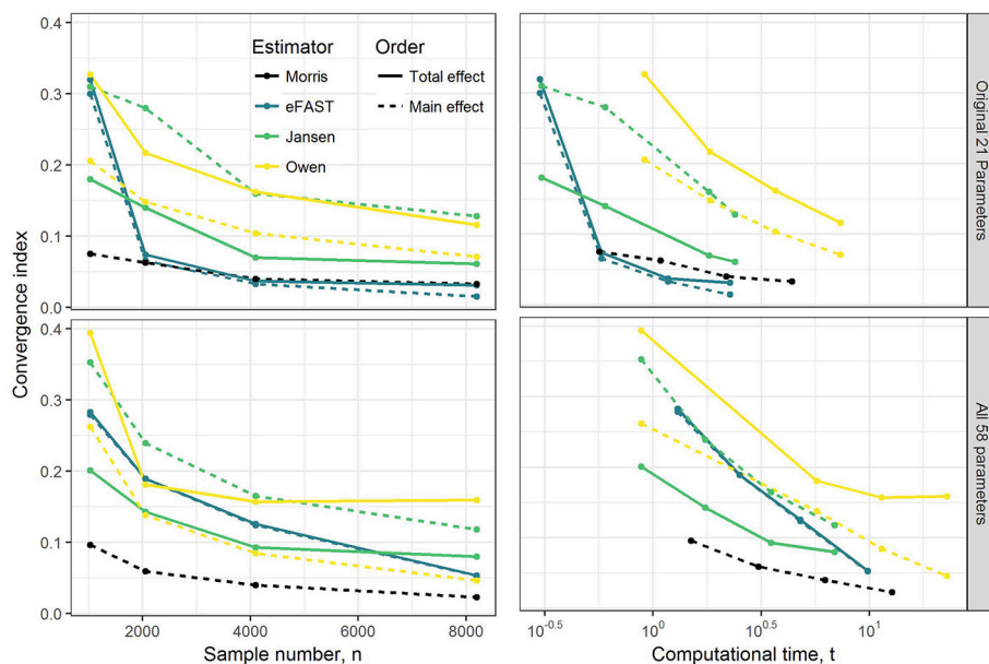
FIGURE 1 | Illustration of the effect of GSA sampling number on convergence index and computational time (min). Note that to check convergence, the sample size has been increased up from 1,024 to 8,192 under OMP and FMP. Each estimated convergence index was based on the model evaluation that was generated from the sample number n .
