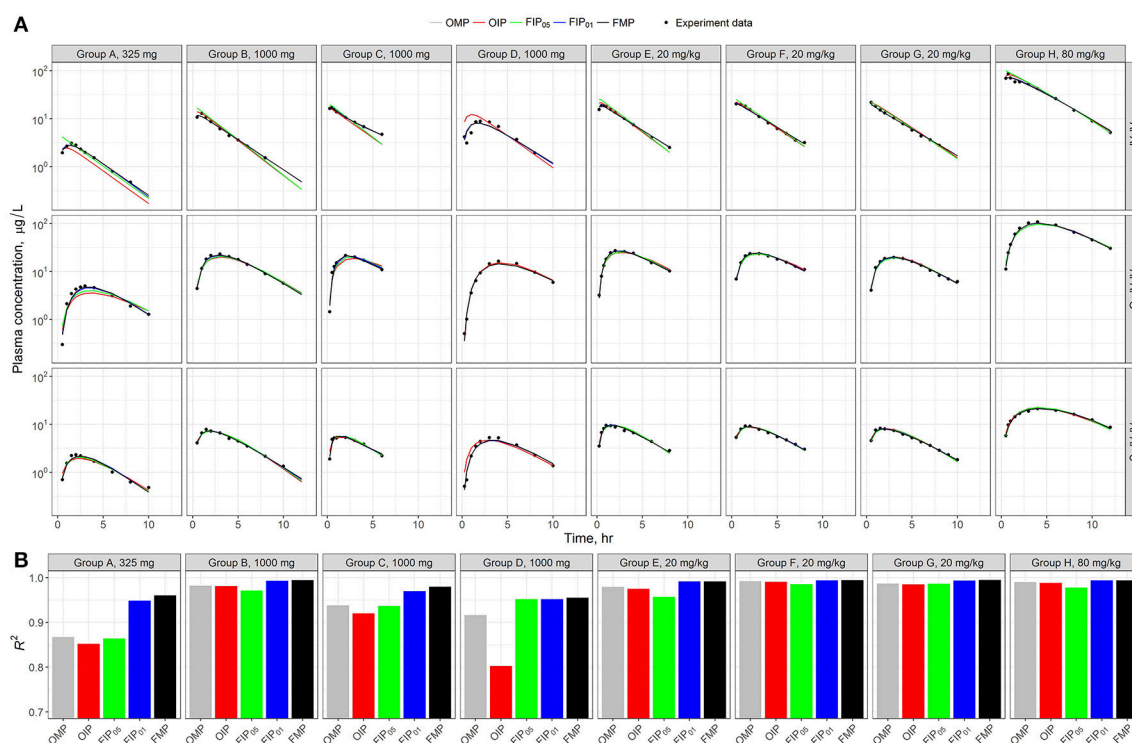
FIGURE 5 | (A) Model evaluation results for the eight experimental human studies with different APAP dosages (Top) across the five parameter sets: original model parameters, OMP (gray); full set of model parameters, FMP (black); 11 original influential parameters, using 0.05 as a cut-off point, OIP (red); full set of 10 influential parameters, using 0.05 as a cut-off point, FIP 05 (green); and full set of 20 influential parameters, using 0.01 as a cut-off point, FIP 01 (blue). (B) The R^2 was used to assess the model performance for each experimental group.
