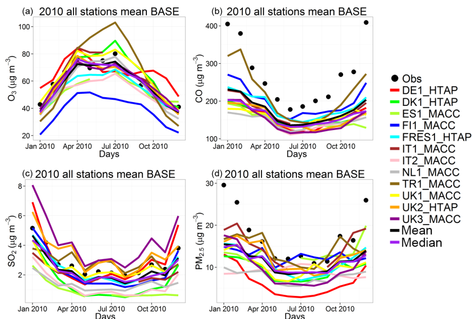
Figure 2. Observed and simulated (base case) monthly (a) \text{O}_3 , (b) \text{CO} , (c) \text{SO}_2 and (d) \text{PM}_{2.5} concentrations over Europe.
