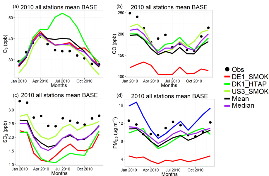
Figure 3. Observed and simulated (base case) monthly (a) \text{O}_3 , (b) \text{CO} , (c) \text{SO}_2 and (d) \text{PM}_{2.5} concentrations over the US.
