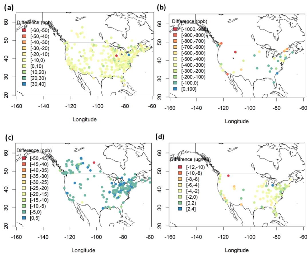
Figure 5. Spatial distribution of annual MM mean bias (ppb for gases and \mu\text{g m}^{-3} for \text{PM}_{2.5} ) for (a) DM8H \text{O}_3 , (b) CO, (c) \text{SO}_2 and (d) \text{PM}_{2.5} over North America.
