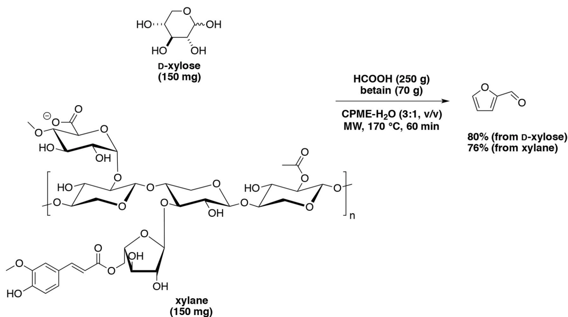
SCHEME 7 | Microwave-assisted production of furfural from D-xylose in the presence of formic acid and betain in a mixture of CPME-H 2 O (Delbecq et al., 2016).
