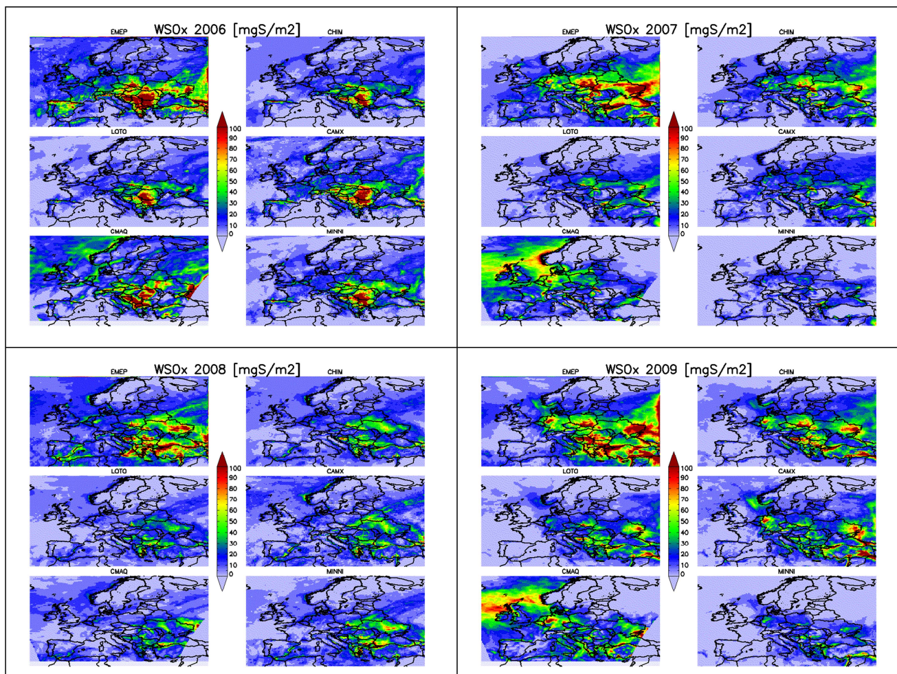
Figure 1. Accumulated deposition maps for WSOx (in mgS/m 2 ), for all the models and periods
