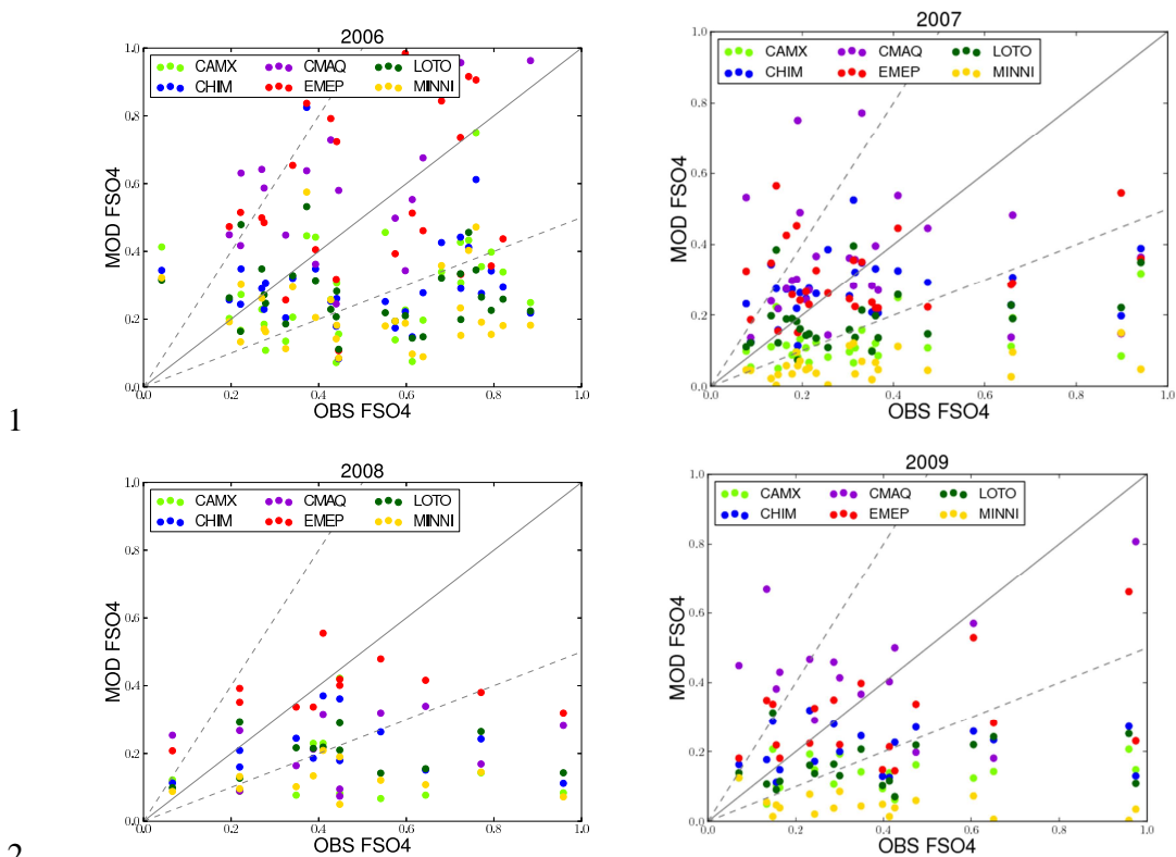
1 2 3 Figure 7. Scatter plots showing modelled and observed FSO4 (not sea salt corrected) (in 4 (\text{mgS}/\text{m}^2)/(\text{ugS}/\text{m}^3)/\text{mm} , for the EMEP intensive campaigns C6, C7, C8, and C9
