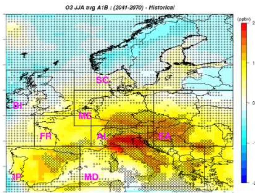
Figure 1 : Increase in surface summertime ozone concentrations (ppbv) by the middle of the century in the moderate climate change scenario A1B in an ensemble of all the published European model projections, [NB. Augustin Colette can make an adapted version if the figure is ultimately selected] (adapted from Colette et al. , 2015a)
