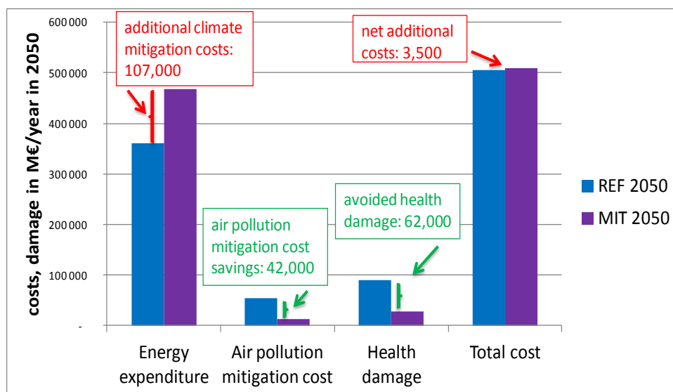
Figure 2 : Win-win strategies: cost benefit analyses at the scale of Europe demonstrate that the additional costs related to climate mitigation (MIT) scenario aiming at a 2°C warming at the end of the century compared to the business as usual scenario (REF) could largely be compensated by savings in end of pipe air pollution mitigation costs and avoided health damages in Europe. Adapted from Schucht et al. , (2015).
