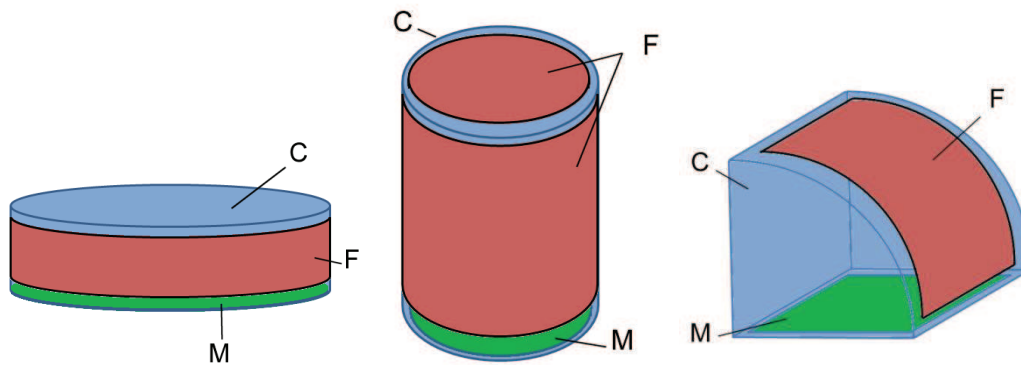
Fig. 1: Three principal types of flameless vents. From left to right: disc, cylinder and box type flameless (M: venting device; C: chamber; F: filter)
