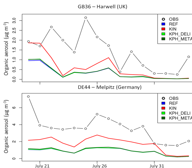
Figure 10. Comparisons of OC measurements (circles) with simulated OC in \text{PM}_{10} obtained in the reference simulation (blue), using the kinetic approach configuration (red), and using both KPH approaches – either in deliquescent or metastable mode (green and dark-green curves, respectively) at the Harwell (UK, top) and Melpitz (Germany, bottom) sites during the month of July 2006.
