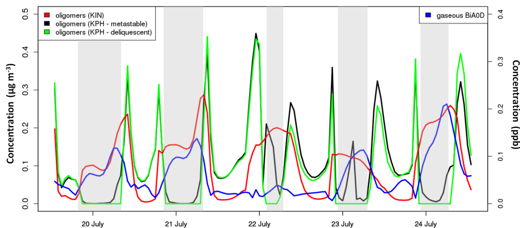
Figure 7. Time series of BiAOD concentrations (ppb) in the reference simulation (blue line), the KIN (red line) oligomer concentrations ( \mu\text{g m}^{-3} ), and the KPH oligomer concentrations ( \mu\text{g m}^{-3} ) in the deliquescent mode (green line) and in the metastable mode (black line), as simulated with CHIMERE for the 20–24 July 2006 period in northern Spain. The shaded areas correspond to the presence of a dry aerosol in the deliquescent configuration.
