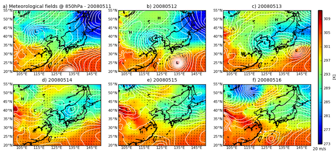
Figure 4. Meteorological situation given at 850 hPa from 11 to 16 May 2008. The coloured areas represent the equivalent potential temperature and the white contours the geopotential height. The “L” and “H” symbols represent the centre of lows and highs respectively. Horizontal winds are also plotted.
