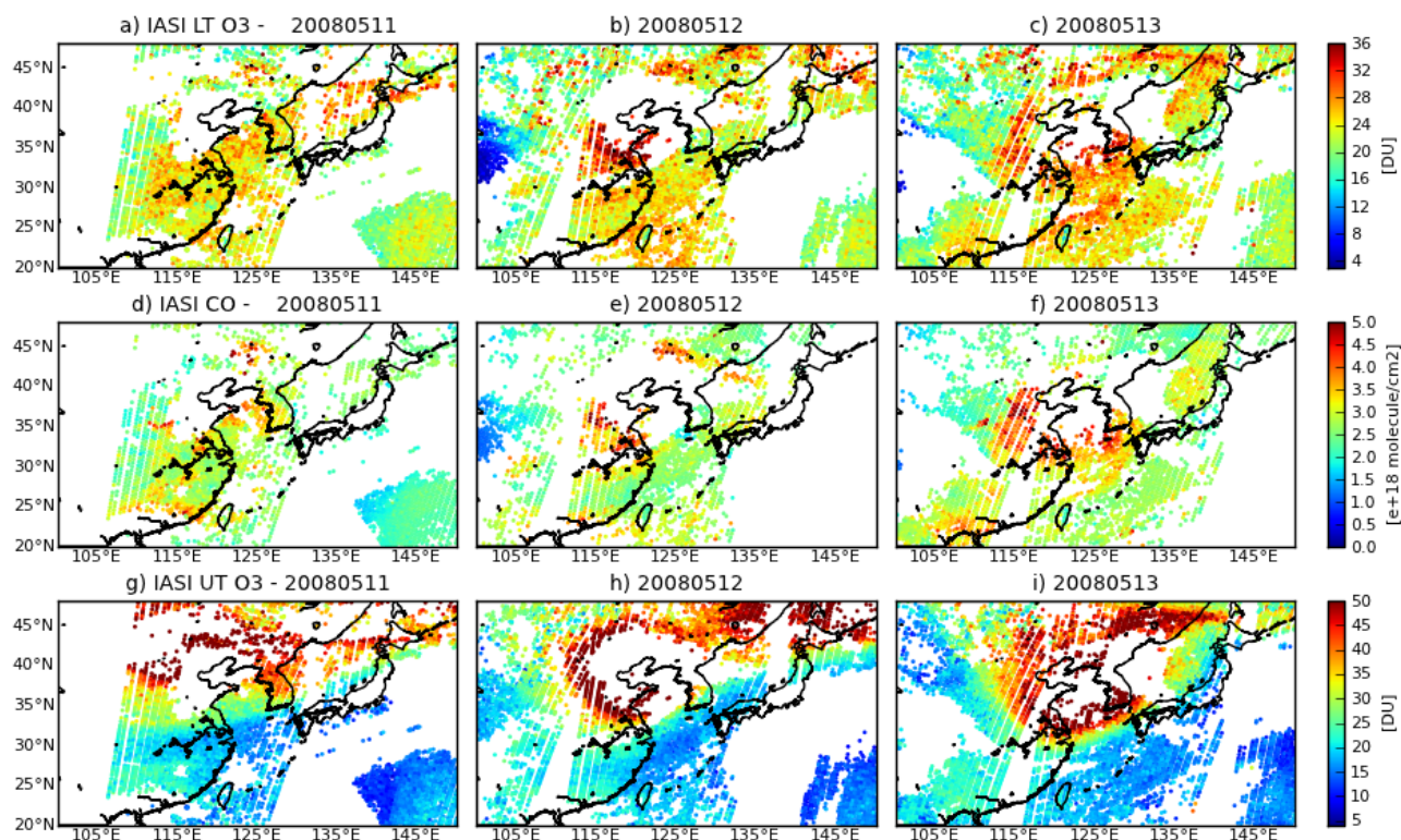
Figure 5. Panels (a–c): lower-tropospheric ozone columns (surface to 6 km a.s.l.) retrieved from IASI from 11 to 13 May 2008. Panels (d–f): total CO columns retrieved from IASI. Panels (g–i): upper-tropospheric ozone columns (6 to 12 km a.s.l.) retrieved from IASI.
