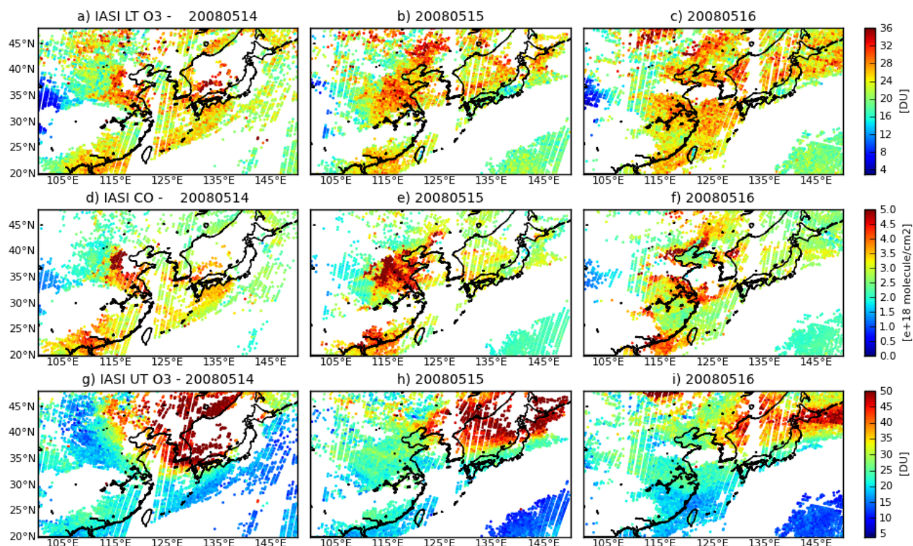
Figure 6. Same as Fig. 5 but for 14 to 16 May 2008.
