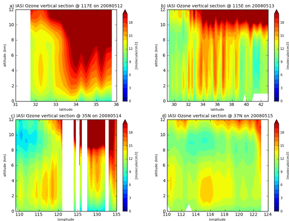
Figure 7. Vertical section of ozone concentration (in molecule \text{cm}^{-3} ) retrieved from IASI along specific longitudes – (a) 117° E on 12 May 2008, (b) 115° E on 13 May 2008 – and along specific latitudes – (c) 35° N on 14 May 2008, (d) 37° N on 15 May 2008. The longitudinal (latitudinal) sections are computed over 1° around the specific longitude (latitude) with a 0.25° resolution in latitude (longitude).
