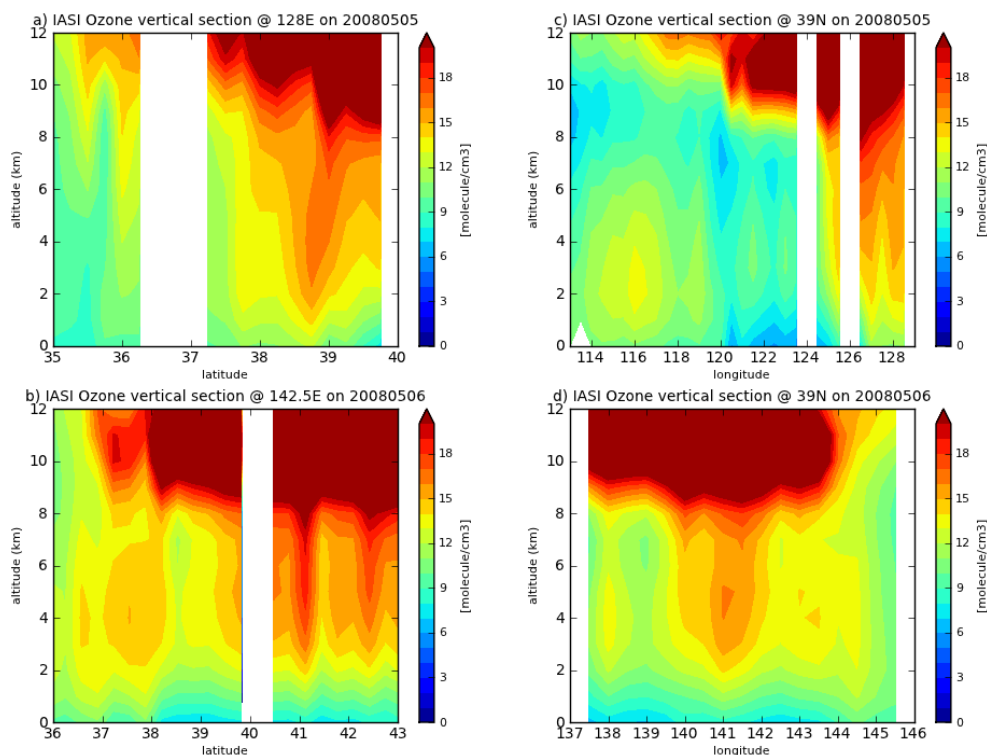
Figure 3. Vertical section of ozone concentration (in molecule \text{cm}^{-3} ) retrieved from IASI along specific longitudes – 128^\circ\text{E} on 5 May 2008 (a), 142.5^\circ\text{E} on 6 May 2008 (b) – and along specific latitudes – 39^\circ\text{N} on 5 May 2008 (c) and 6 May 2008 (d). The longitudinal (latitudinal) sections are computed over 1^\circ around the specific longitude (latitude) with a 0.25^\circ resolution in latitude (longitude).
