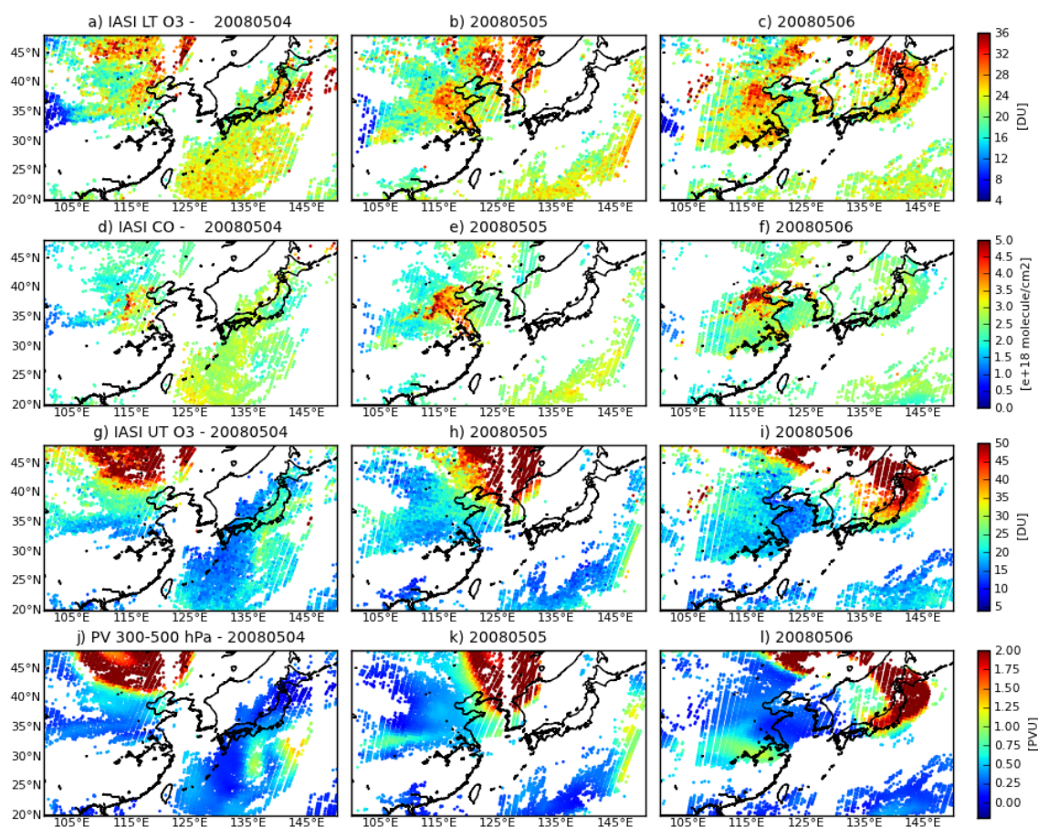
Figure 2. Panels (a–c): lower-tropospheric ozone columns (surface to 6 km a.s.l.) retrieved from IASI from 4 to 6 May 2008; panels (d–f): total CO columns retrieved from IASI; panels (g–i): upper-tropospheric ozone columns (6 to 12 km a.s.l.) retrieved from IASI; panels (j–l): potential vorticity (PV) from ERA5 Interim reanalysis averaged between 300 and 500 hPa.
