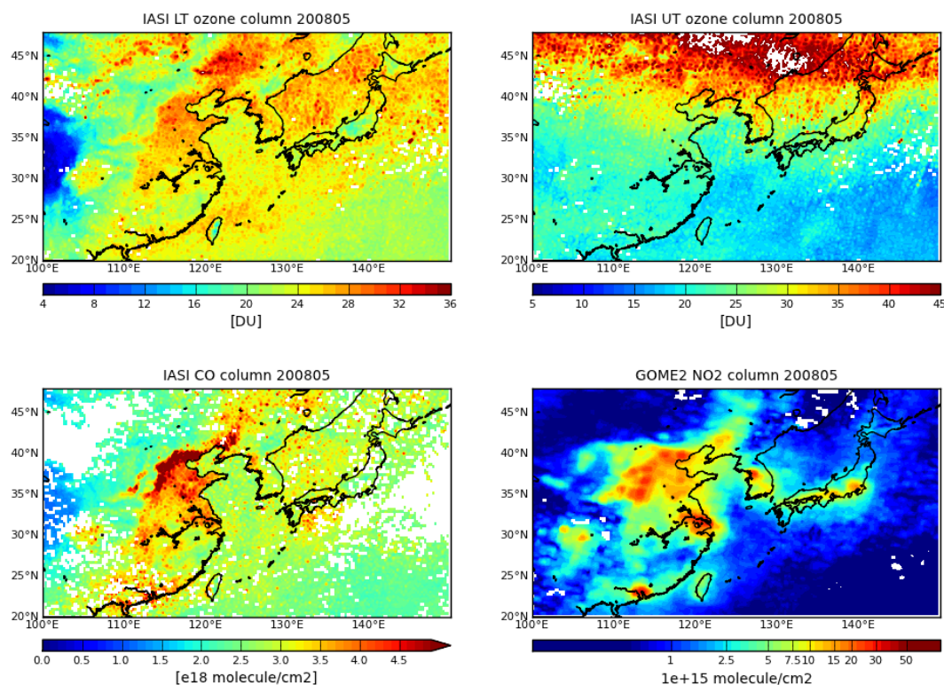
Figure 9. Monthly lower (upper left) and upper (upper right) tropospheric ozone columns observed by IASI in May 2008 as well as monthly IASI total CO columns (lower left) and GOME-2 NO 2 tropospheric columns (lower right) observed in May 2008. The average is calculated for a 0.25^\circ \times 0.25^\circ resolution grid.
