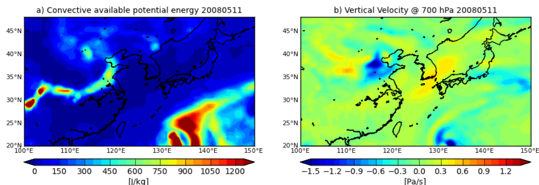
Figure 8. Convective available potential energy (a) and vertical velocity at 700 hPa (b) from ERA-Interim reanalysis.
