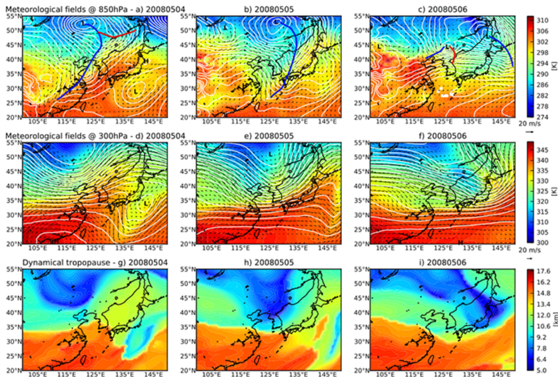
Figure 1. Meteorological situation given at (a–c) 850 hPa and (d–f) 300 hPa from 4 to 6 May 2008 as well as (g–i) the dynamical tropopause. All the meteorological variables are derived from the ERA-Interim reanalysis. The coloured areas in (a–f) represent the equivalent potential temperature and the white contours the geopotential height. The “L” and “H” symbols represent the centre of lows and highs respectively. Horizontal winds are also plotted. The cold and warm fronts are displayed in blue and red respectively on the top panel.
