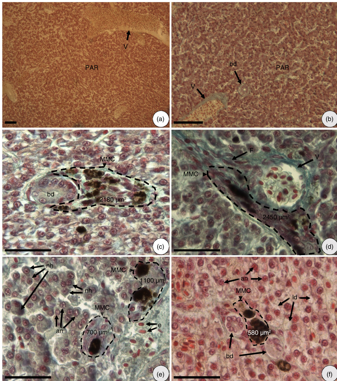
Fig. 3 Photomicrographs of liver sections from brown trout from the Kerguelen Islands illustrating (a, b) normal parenchyma. (c–f) Important numbers of melanomacrophage centres (MMC). The following terms are abbreviated: parenchyma (PAR), vein (V), biliary duct (bd); MMC; fibrosis (F), necrotic hepatocyte (nh); altered nucleus (an); erythrocyte (e), lipidic droplet (ld). The dotted line represents the MMC boundary. The scale bars are 40 \mu\text{m} in length.
